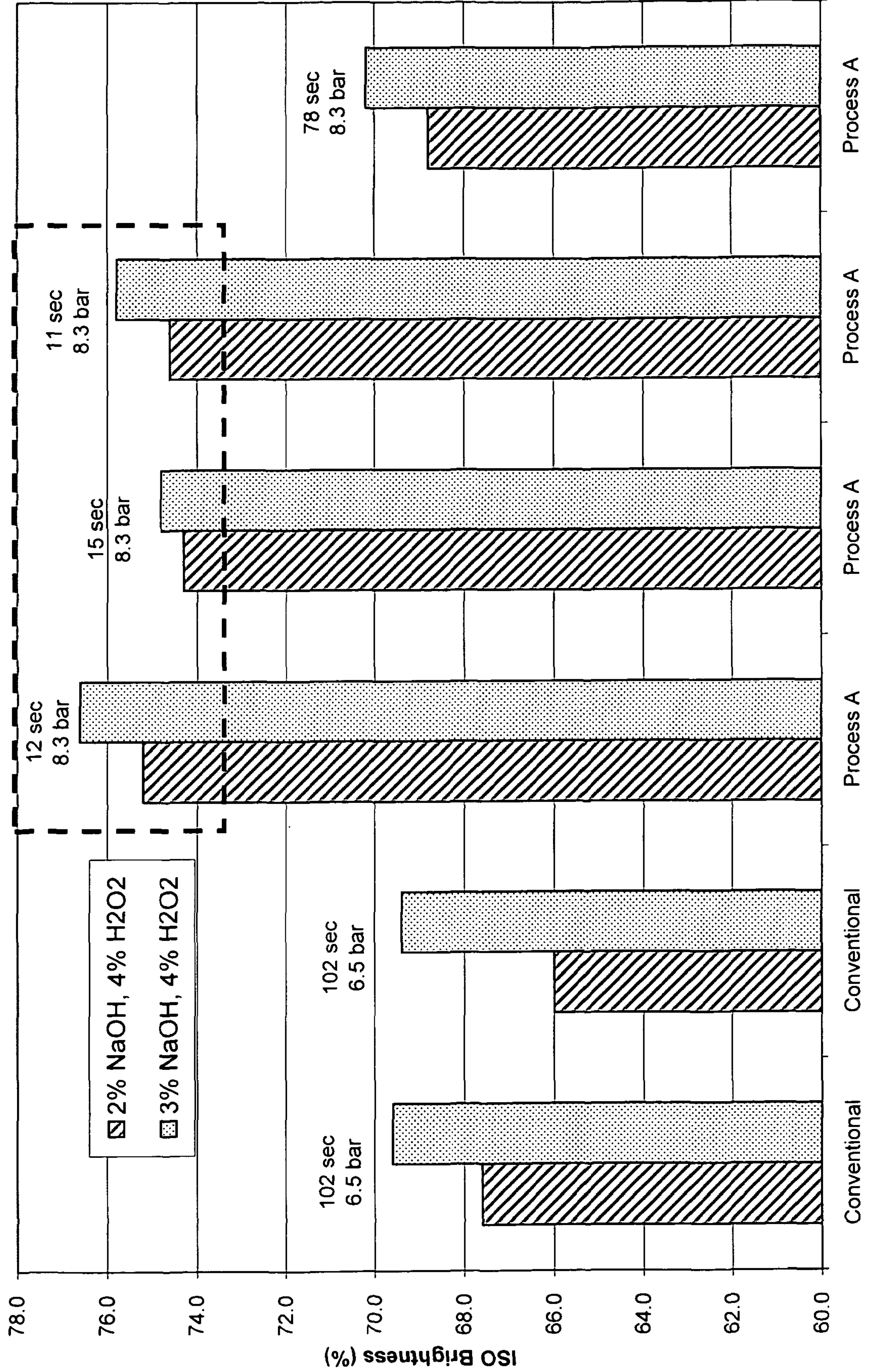
Figure 13: Bleached Brightness
