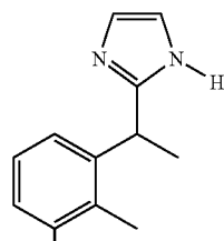
Demiditraz racemate (Pfizer)
