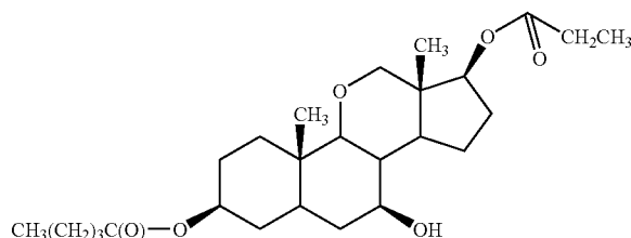
group 27-11-1 compound 1.2.5.9
