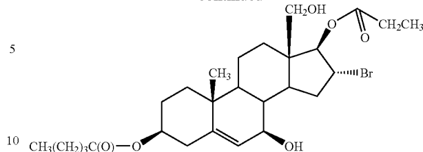
group 11-8-2 compound 1.2.1.9.
