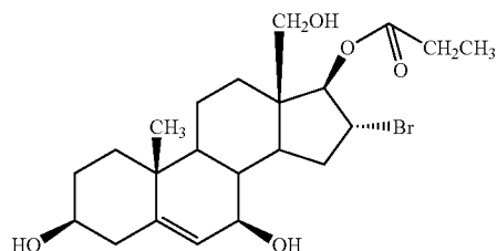
group 8-2 compound 1.2.1.9.
