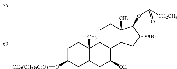
group 11-1 compound 1.2.1.9
