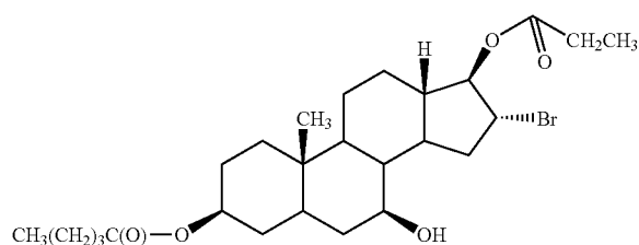
group 11-7-1 compound 1.2.1.9.
