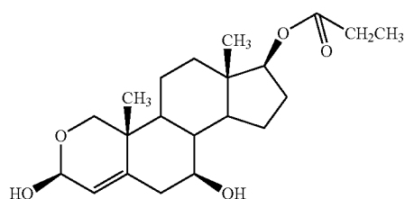
group 28-5 compound 1.2.5.9.
