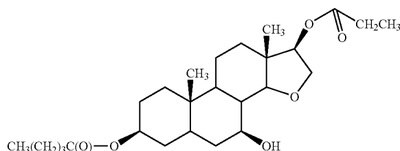
group 26-11-1 compound 1.2.5.9
