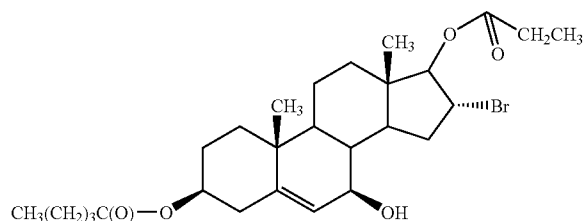
group 11-2 compound 1.2.1.9.
