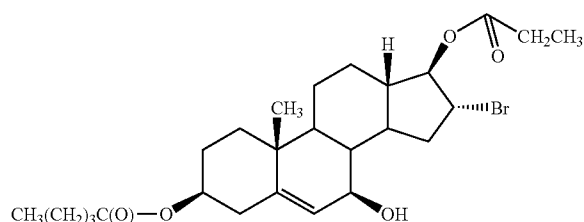
group 11-7-2 compound 1.2.1.9.
