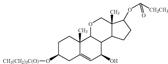
group 27-11-1 compound 1.2.5.9
