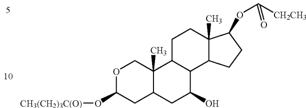
group 28-11-1 compound 1.2.5.9
