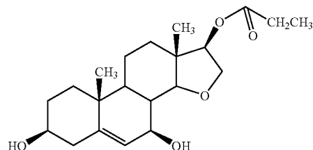
group 26-2 compound 1.2.5.9.
