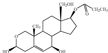
group 28-8-2 compound 1.2.5.9.
