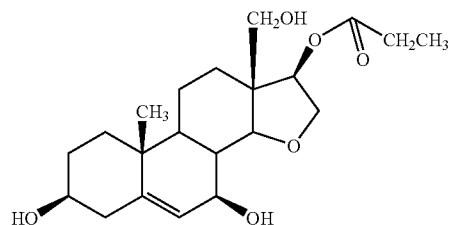
group 26-8-2 compound 1.2.5.9.
