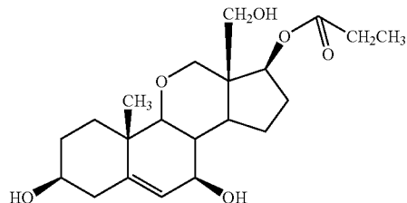
group 27-8-2 compound 1.2.5.9.
