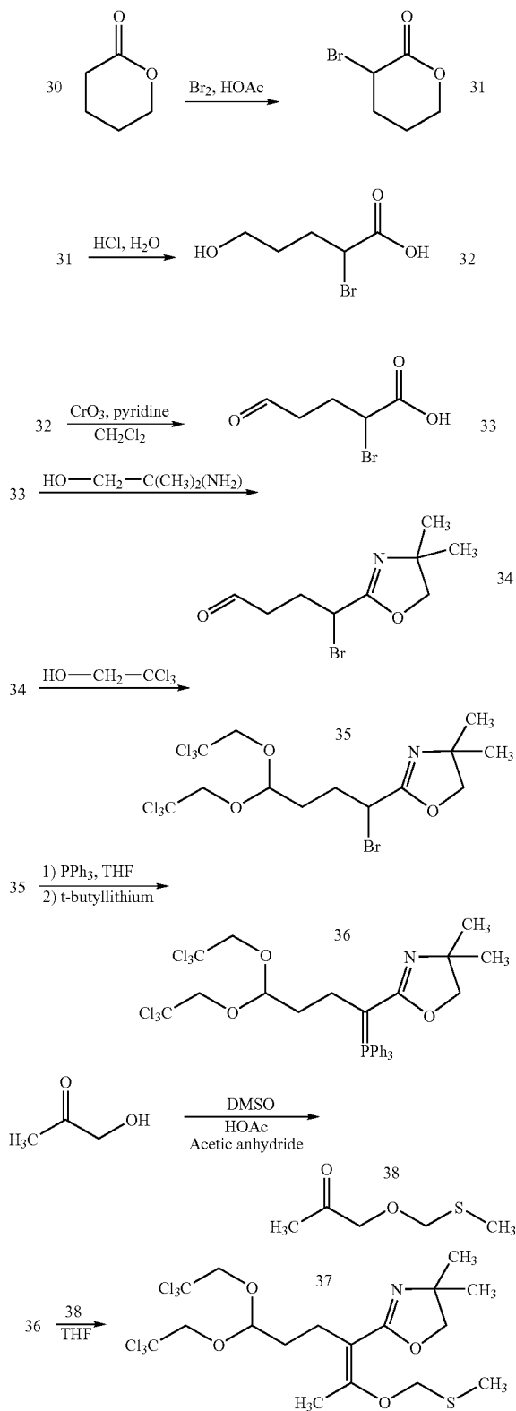
Scheme 12A
