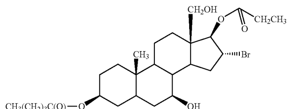
group 11-8-1 compound 1.2.1.9.
