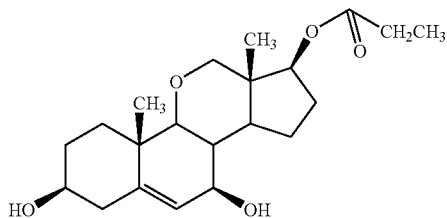
group 27-2 compound 1.2.5.9.
