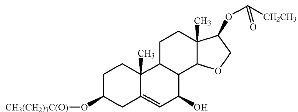
group 26-11-2 compound 1.2.5.9.
