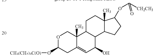
group 28-11-1 compound 1.2.5.9
