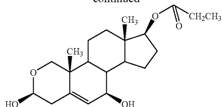
group 28-2 compound 1.2.5.9.
