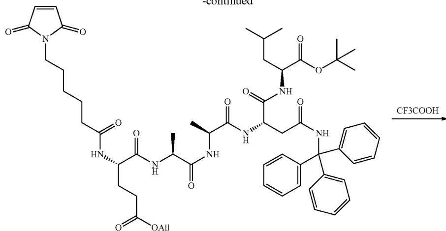
Intermediate 7
