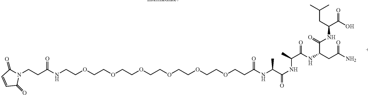
Intermediate 8
