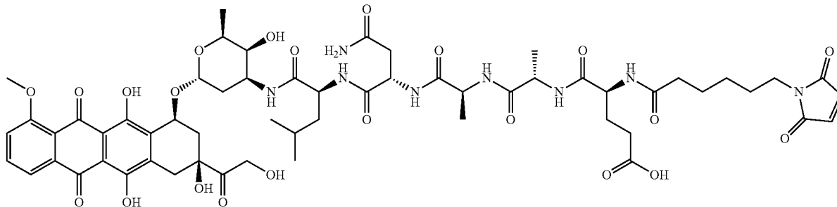
Intermediate 9
