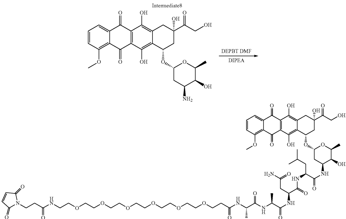
Intermediate 8
