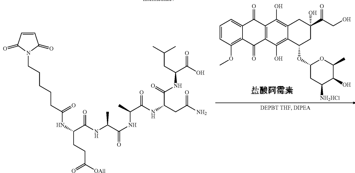
Intermediate 8
