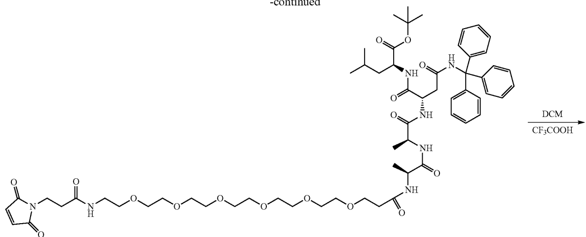
Intermediate 7
