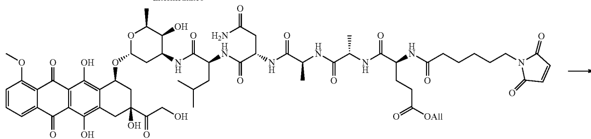
Intermediate 9
