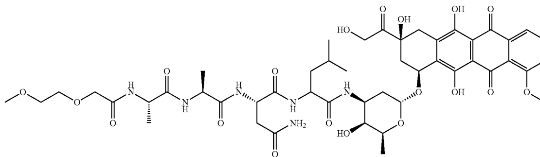
PEG-AANL-DOX
