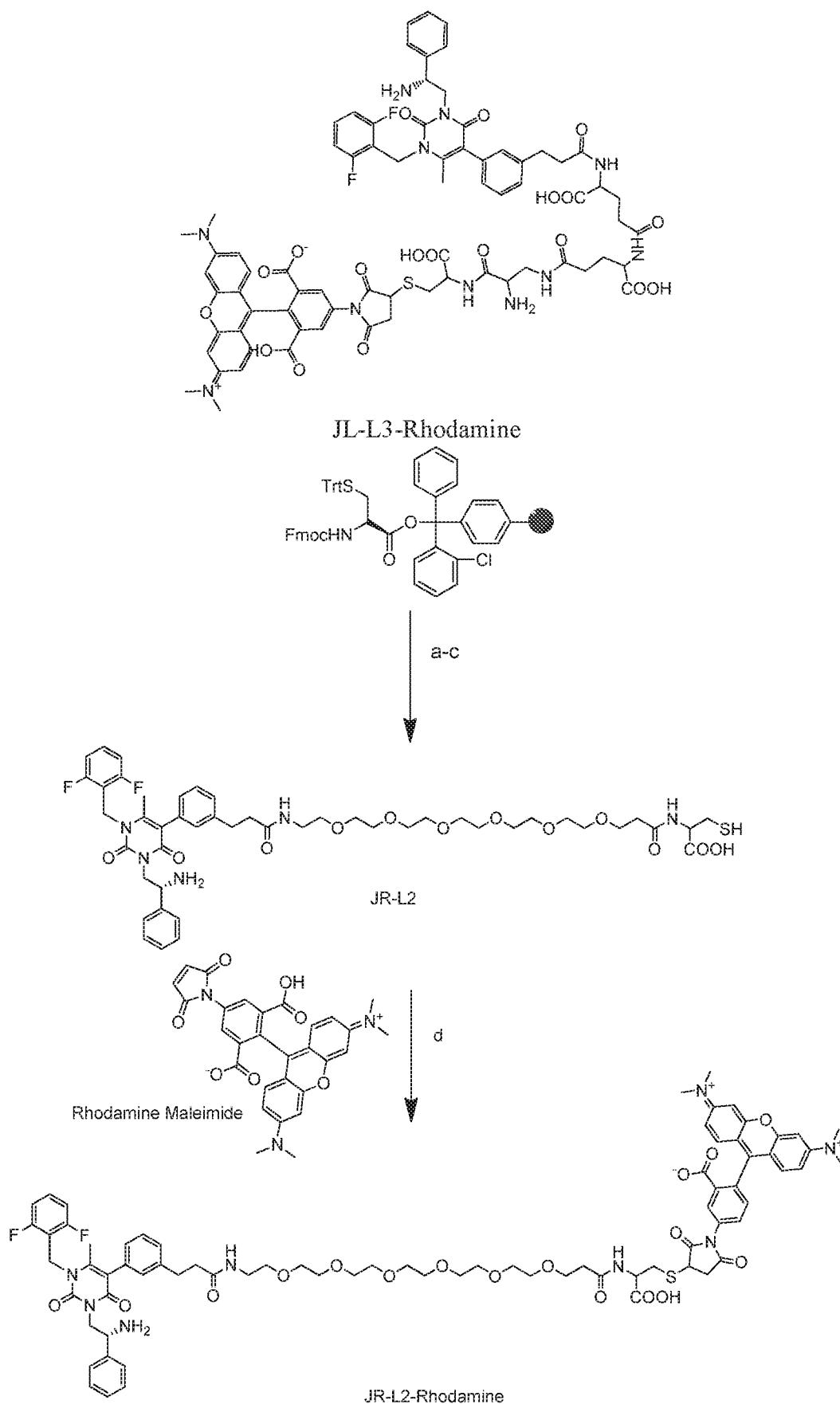
[00359] Scheme 7. Synthesis of JR-L2-Rhodamine, Reagents and conditions: (a) (i) 20% piperidine/DMF, rt, (ii) Fmoc-N-amido-dPEG 6 -acid, PyBop, DMF, DIPEA, (b) (i) 20%
