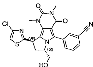
3-((7S,9R)-9-(4-chlorothiazol-2-yl)-7-(hydroxymethyl)-1,3-dimethyl-2,4-dioxo-2,3,4,7,8,9-hexahydro-1H-pyrimido[4,5-a]pyrrolizin-5-yl)benzonitrile
