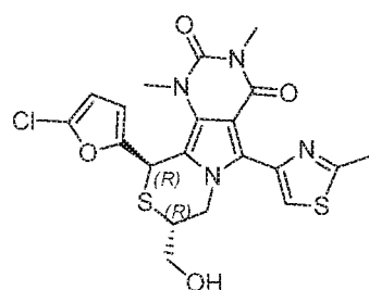
(8R,10R)-10-(5-chlorofuran-2-yl)-8-(hydroxymethyl)-1,3-dimethyl-5-(2-methylthiazol-4-yl)-7,8-dihydro-1H-pyrimido[4',5':3,4]pyrrolo[2,1-c][1,4]thiazine-2,4(3H,10H)-dione
