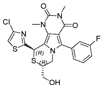
(8 R ,10 R )-10-(4-chlorothiazol-2-yl)-5-(3-fluorophenyl)-8-(hydroxymethyl)-1,3-dimethyl-7,8-dihydro-1 H -pyrimido[4',5':3,4]pyrrolo[2,1-c][1,4]thiazine-2,4(3 H ,10 H )-dione
