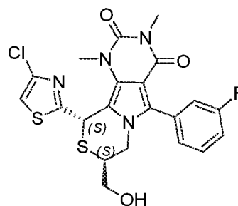
(8 S ,10 S )-10-(4-chlorothiazol-2-yl)-5-(3-fluorophenyl)-8-(hydroxymethyl)-1,3-dimethyl-7,8-dihydro-1 H -pyrimido[4',5':3,4]pyrrolo[2,1- c ][1,4]thiazine-2,4(3 H ,10 H )-dione
