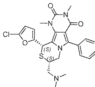
(8 S ,10 S )-10-(5-chlorofuran-2-yl)-8-((dimethylamino)methyl)-1,3-dimethyl-5-phenyl-7,8-dihydro-1 H -pyrimido[4',5':3,4]pyrrolo[2,1- c ][1,4]thiazine-2,4(3 H ,10 H )-dione
