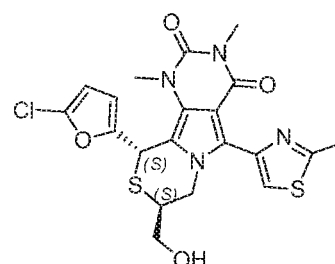
(8S,10S)-10-(5-chlorofuran-2-yl)-8-(hydroxymethyl)-1,3-dimethyl-5-(2-methylthiazol-4-yl)-7,8-dihydro-1H-pyrimido[4',5':3,4]pyrrolo[2,1-c][1,4]thiazine-2,4(3H,10H)-dione
