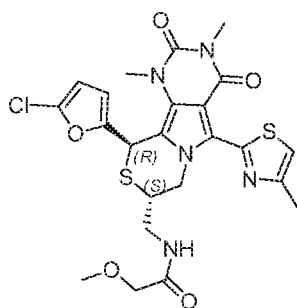
N-(((8S,10R)-10-(5-chlorofuran-2-yl)-1,3-dimethyl-5-(4-methylthiazol-2-yl)-2,4-dioxo-2,3,4,7,8,10-hexahydro-1H-pyrimido[4',5':3,4]pyrrolo[2,1-c][1,4]thiazin-8-yl)methyl)-2-methoxyacetamide
