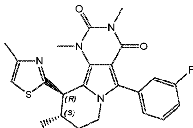
(9S,10R)-5-(3-fluorophenyl)-1,3,9-trimethyl-10-(4-methylthiazol-2-yl)-7,8,9,10-tetrahydropyrimido[4,5-a]indolizine-2,4(1H,3H)-dione
