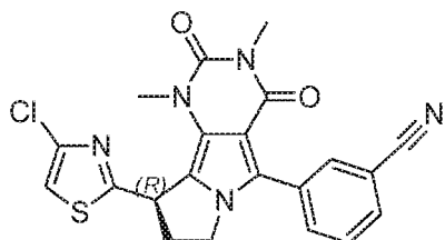
(R)-3-(9-(4-chlorothiazol-2-yl)-1,3-dimethyl-2,4-dioxo-2,3,4,7,8,9-hexahydro-1H-pyrimido[4,5-a]pyrrolizin-5-yl)benzonitrile
