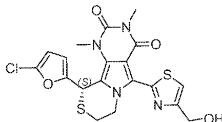
(S)-10-(5-chlorofuran-2-yl)-5-(4-(hydroxymethyl)thiazol-2-yl)-1,3-dimethyl-7,8-dihydro-1H-pyrimido[4',5':3,4]pyrrolo[2,1-c][1,4]thiazine-2,4(3H,10H)-dione
