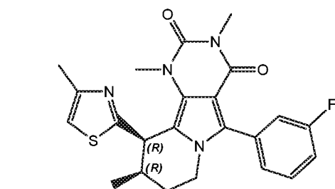
(9R,10R)-5-(3-fluorophenyl)-1,3,9-trimethyl-10-(4-methylthiazol-2-yl)-7,8,9,10-tetrahydropyrimido[4,5-a]indolizine-2,4(1H,3H)-dione
