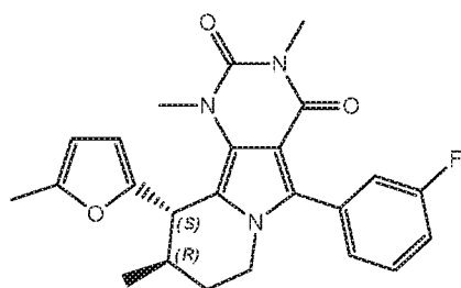
(9 R ,10 S )-5-(3-fluorophenyl)-1,3,9-trimethyl-10-(5-methylfuran-2-yl)-7,8,9,10-tetrahydropyrimido[4,5- a ]indolizine-2,4(1 H ,3 H )-dione
