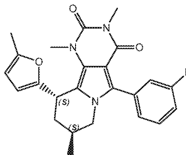
(8S,10S)-5-(3-fluorophenyl)-1,3,8-trimethyl-10-(5-methylfuran-2-yl)-7,8,9,10-tetrahydropyrimido[4,5-a]indolizine-2,4(1H,3H)-dione
