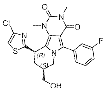
(8 S ,10 R )-10-(4-chlorothiazol-2-yl)-5-(3-fluorophenyl)-8-(hydroxymethyl)-1,3-dimethyl-7,8,9,10-tetrahydropyrimido[4,5- a ]indolizine-2,4(1 H ,3 H )-dione
