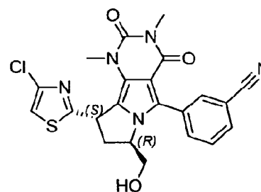
3-((7R,9S)-9-(4-chlorothiazol-2-yl)-7-(hydroxymethyl)-1,3-dimethyl-2,4-dioxo-2,3,4,7,8,9-hexahydro-1H-pyrimido[4,5-a]pyrrolizin-5-yl)benzonitrile
