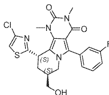
(8 S ,10 S )-10-(4-chlorothiazol-2-yl)-5-(3-fluorophenyl)-8-(hydroxymethyl)-1,3-dimethyl-7,8,9,10-tetrahydropyrimido[4,5- a ]indolizine-2,4(1 H ,3 H )-dione
