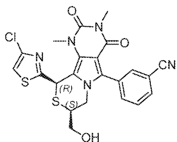
3-((8 S ,10 R )-10-(4-chlorothiazol-2-yl)-8-(hydroxymethyl)-1,3-dimethyl-2,4-dioxo-2,3,4,7,8,10-hexahydro-1 H -pyrimido[4',5':3,4]pyrrolo[2,1- c ][1,4]thiazin-5-yl)benzonitrile
