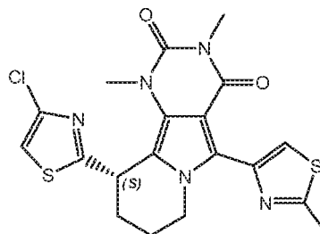
( S )-10-(4-chlorothiazol-2-yl)-1,3-dimethyl-5-(2-methylthiazol-4-yl)-7,8,9,10-tetrahydropyrimido[4,5- a ]indolizine-2,4(1 H ,3 H )-dione
