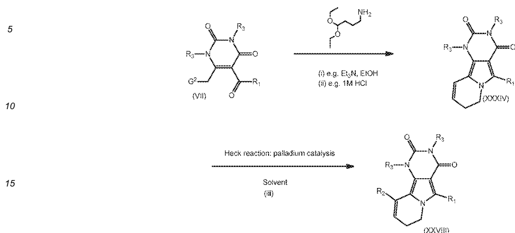
Scheme 9
