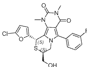
(8 S ,10 S )-10-(5-chlorofuran-2-yl)-5-(3-fluorophenyl)-8-(hydroxymethyl)-1,3-dimethyl-7,8-dihydro-1 H -pyrimido[4',5':3,4]pyrrolo[2,1- c ][1,4]thiazine-2,4(3 H ,10 H )-dione
