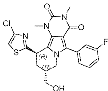
(8 R ,10 R )-10-(4-chlorothiazol-2-yl)-5-(3-fluorophenyl)-8-(hydroxymethyl)-1,3-dimethyl-7,8,9,10-tetrahydropyrimido[4,5- a ]indolizine-2,4(1 H ,3 H )-dione
