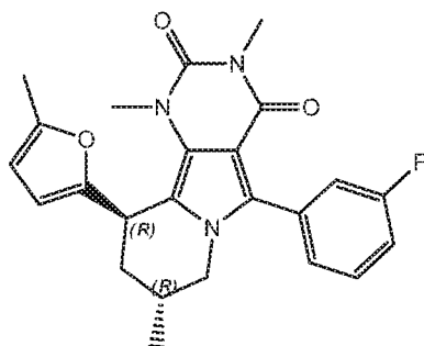
(8R,10R)-5-(3-fluorophenyl)-1,3,8-trimethyl-10-(5-methylfuran-2-yl)-7,8,9,10-tetrahydropyrimido[4,5-a]indolizine-2,4(1H,3H)-dione
