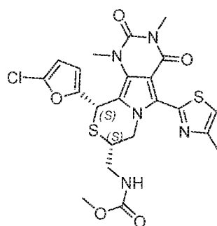
methyl (((8S,10S)-10-(5-chlorofuran-2-yl)-1,3-dimethyl-5-(4-methylthiazol-2-yl)-2,4-dioxo-2,3,4,7,8,10-hexahydro-1H-pyrimido[4',5':3,4]pyrrolo[2,1-c][1,4]thiazin-8-yl)methyl)carbamate
