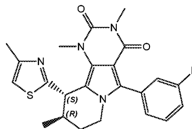
(9R,10S)-5-(3-fluorophenyl)-1,3,9-trimethyl-10-(4-methylthiazol-2-yl)-7,8,9,10-tetrahydropyrimido[4,5-a]indolizine-2,4(1H,3H)-dione
