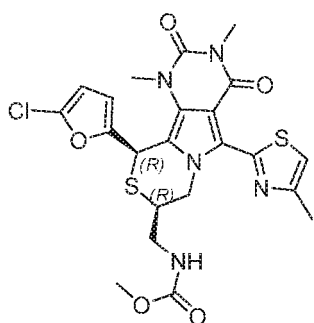
methyl (((8R,10R)-10-(5-chlorofuran-2-yl)-1,3-dimethyl-5-(4-methylthiazol-2-yl)-2,4-dioxo-2,3,4,7,8,10-hexahydro-1H-pyrimido[4',5':3,4]pyrrolo[2,1-c][1,4]thiazin-8-yl)methyl)carbamate
