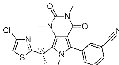
(S)-3-(9-(4-chlorothiazol-2-yl)-1,3-dimethyl-2,4-dioxo-2,3,4,7,8,9-hexahydro-1H-pyrimido[4,5-a]pyrrolizin-5-yl)benzonitrile
