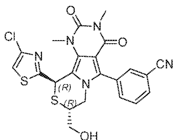
3-((8 R ,10 R )-10-(4-chlorothiazol-2-yl)-8-(hydroxymethyl)-1,3-dimethyl-2,4-dioxo-2,3,4,7,8,10-hexahydro-1 H -pyrimido[4',5':3,4]pyrrolo[2,1- c ][1,4]thiazin-5-yl)benzonitrile
