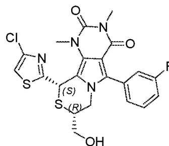
(8 R ,10 S )-10-(4-chlorothiazol-2-yl)-5-(3-fluorophenyl)-8-(hydroxymethyl)-1,3-dimethyl-7,8-dihydro-1 H -pyrimido[4',5':3,4]pyrrolo[2,1-c][1,4]thiazine-2,4(3 H ,10 H )-dione
