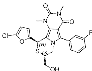
(8 S ,10 R )-10-(5-chlorofuran-2-yl)-5-(3-fluorophenyl)-8-(hydroxymethyl)-1,3-dimethyl-7,8-dihydro-1 H -pyrimido[4',5':3,4]pyrrolo[2,1- c ][1,4]thiazine-2,4(3 H ,10 H )-dione
