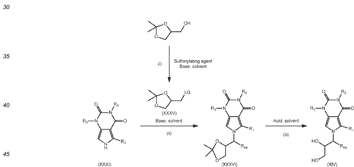
Scheme 10
