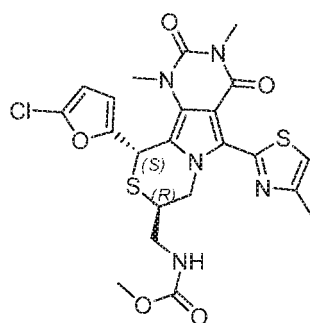
methyl (((8R,10S)-10-(5-chlorofuran-2-yl)-1,3-dimethyl-5-(4-methylthiazol-2-yl)-2,4-dioxo-2,3,4,7,8,10-hexahydro-1H-pyrimido[4',5':3,4]pyrrolo[2,1-c][1,4]thiazin-8-yl)methyl)carbamate
