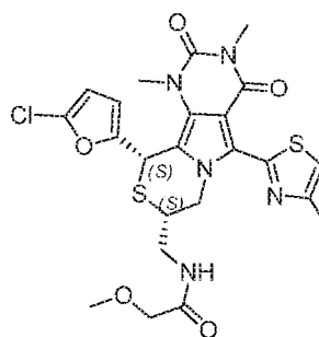
N-(((8S,10S)-10-(5-chlorofuran-2-yl)-1,3-dimethyl-5-(4-methylthiazol-2-yl)-2,4-dioxo-2,3,4,7,8,10-hexahydro-1H-pyrimido[4',5':3,4]pyrrolo[2,1-c][1,4]thiazin-8-yl)methyl)-2-methoxyacetamide
