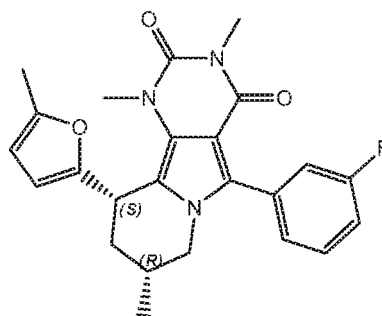
(8R,10S)-5-(3-fluorophenyl)-1,3,8-trimethyl-10-(5-methylfuran-2-yl)-7,8,9,10-tetrahydropyrimido[4,5-a]indolizine-2,4(1H,3H)-dione
