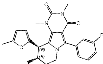
(9 R ,10 R )-5-(3-fluorophenyl)-1,3,9-trimethyl-10-(5-methylfuran-2-yl)-7,8,9,10-tetrahydropyrimido[4,5- a ]indolizine-2,4(1 H ,3 H )-dione
