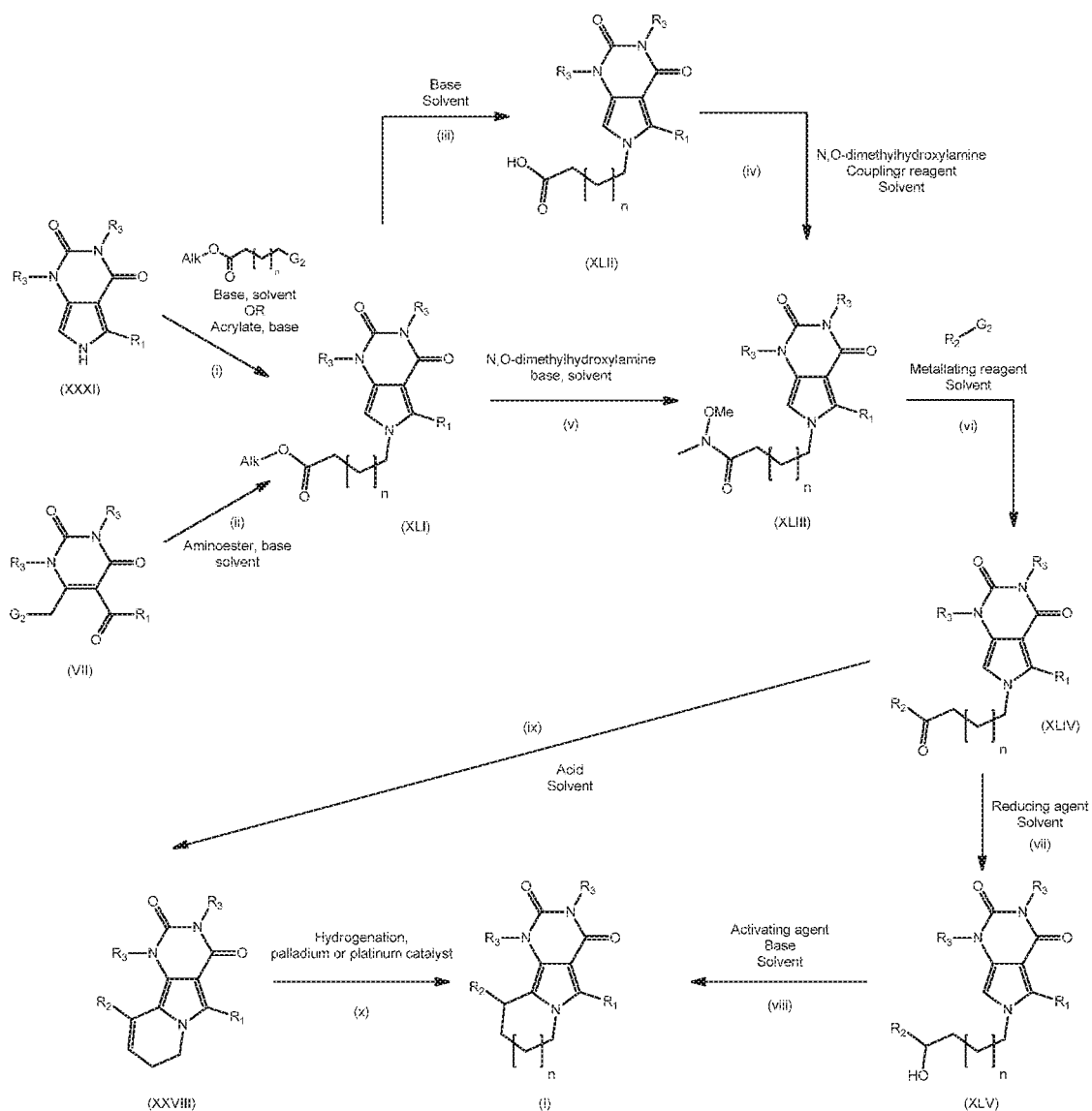
Scheme 13
