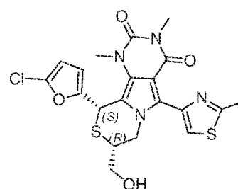
(8R,10S)-10-(5-chlorofuran-2-yl)-8-(hydroxymethyl)-1,3-dimethyl-5-(2-methylthiazol-4-yl)-7,8-dihydro-1H-pyrimido[4',5':3,4]pyrrolo[2,1-c][1,4]thiazine-2,4(3H,10H)-dione
