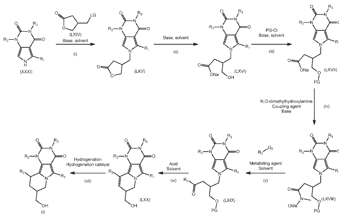
Scheme 19
