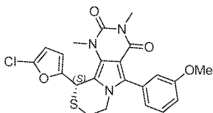
(S)-10-(5-chlorofuran-2-yl)-5-(3-methoxyphenyl)-1,3-dimethyl-7,8-dihydro-1H-pyrimido[4',5':3,4]pyrrolo[2,1-c][1,4]thiazine-2,4(3H,10H)-dione
