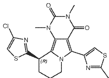
( R )-10-(4-chlorothiazol-2-yl)-1,3-dimethyl-5-(2-methylthiazol-4-yl)-7,8,9,10-tetrahydropyrimido[4,5- a ]indolizine-2,4(1 H ,3 H )-dione
