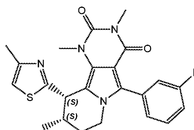
(9S,10S)-5-(3-fluorophenyl)-1,3,9-trimethyl-10-(4-methylthiazol-2-yl)-7,8,9,10-tetrahydropyrimido[4,5-a]indolizine-2,4(1H,3H)-dione
