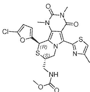
methyl (((8S,10R)-10-(5-chlorofuran-2-yl)-1,3-dimethyl-5-(4-methylthiazol-2-yl)-2,4-dioxo-2,3,4,7,8,10-hexahydro-1H-pyrimido[4',5':3,4]pyrrolo[2,1-c][1,4]thiazin-8-yl)methyl)carbamate
