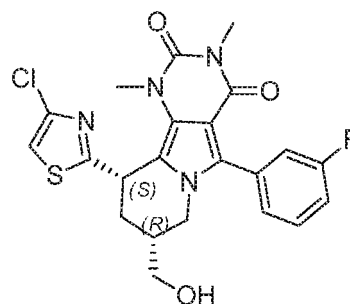
(8 R ,10 S )-10-(4-chlorothiazol-2-yl)-5-(3-fluorophenyl)-8-(hydroxymethyl)-1,3-dimethyl-7,8,9,10-tetrahydropyrimido[4,5- a ]indolizine-2,4(1 H ,3 H )-dione
