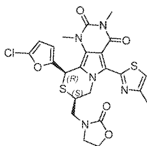
(8 S ,10 R )-10-(5-chlorofuran-2-yl)-1,3-dimethyl-5-(4-methylthiazol-2-yl)-8-((2-oxooxazolidin-3-yl)methyl)-7,8-dihydro-1 H -pyrimido[4',5':3,4]pyrrolo[2,1- c ][1,4]thiazine-2,4(3 H ,10 H )-dione
