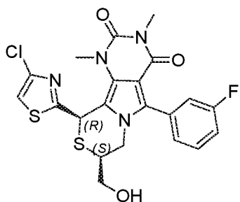
(8 S ,10 R )-10-(4-chlorothiazol-2-yl)-5-(3-fluorophenyl)-8-(hydroxymethyl)-1,3-dimethyl-7,8-dihydro-1 H -pyrimido[4',5':3,4]pyrrolo[2,1- c ][1,4]thiazine-2,4(3 H ,10 H )-dione
