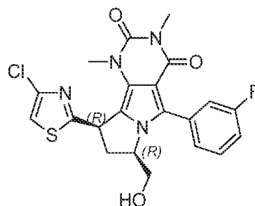
(7 R ,9 R )-9-(4-chlorothiazol-2-yl)-5-(3-fluorophenyl)-7-(hydroxymethyl)-1,3-dimethyl-8,9-dihydro-1 H -pyrimido[4,5- a ]pyrrolizine-2,4(3 H ,7 H )-dione
