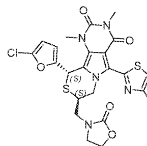
(8 S ,10 S )-10-(5-chlorofuran-2-yl)-1,3-dimethyl-5-(4-methylthiazol-2-yl)-8-((2-oxooxazolidin-3-yl)methyl)-7,8-dihydro-1 H -pyrimido[4',5':3,4]pyrrolo[2,1- c ][1,4]thiazine-2,4(3 H ,10 H )-dione
