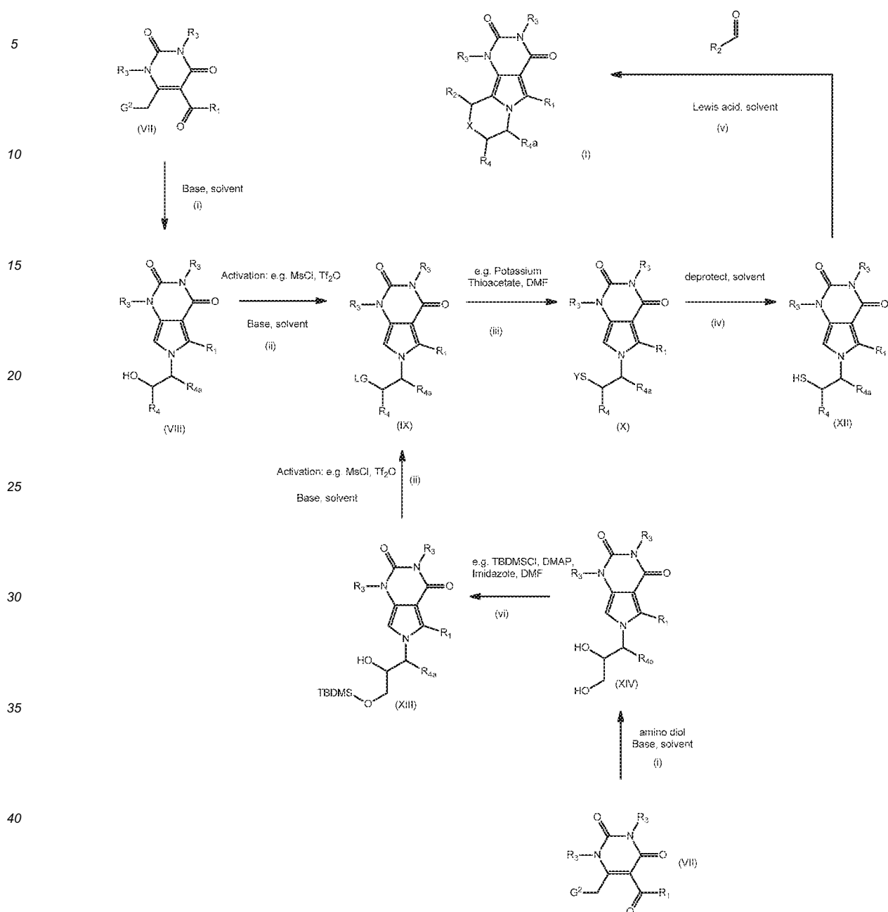
Scheme 3
