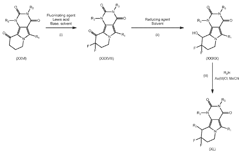
Scheme 12
