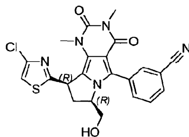
3-((7R,9R)-9-(4-chlorothiazol-2-yl)-7-(hydroxymethyl)-1,3-dimethyl-2,4-dioxo-2,3,4,7,8,9-hexahydro-1H-pyrimido[4,5-a]pyrrolizin-5-yl)benzonitrile
