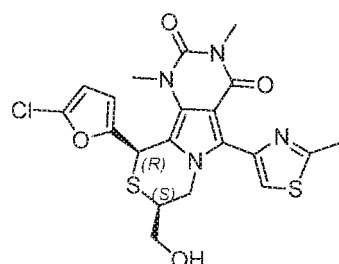
(8S,10R)-10-(5-chlorofuran-2-yl)-8-(hydroxymethyl)-1,3-dimethyl-5-(2-methylthiazol-4-yl)-7,8-dihydro-1H-pyrimido[4',5':3,4]pyrrolo[2,1-c][1,4]thiazine-2,4(3H,10H)-dione
