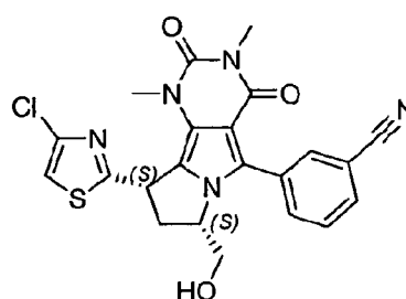
3-((7S,9S)-9-(4-chlorothiazol-2-yl)-7-(hydroxymethyl)-1,3-dimethyl-2,4-dioxo-2,3,4,7,8,9-hexahydro-1H-pyrimido[4,5-a]pyrrolizin-5-yl)benzonitrile
