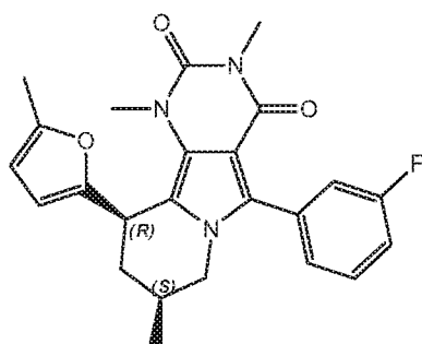
(8S,10R)-5-(3-fluorophenyl)-1,3,8-trimethyl-10-(5-methylfuran-2-yl)-7,8,9,10-tetrahydropyrimido[4,5-a]indolizine-2,4(1H,3H)-dione
