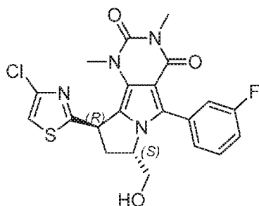
(7 S ,9 R )-9-(4-chlorothiazol-2-yl)-5-(3-fluorophenyl)-7-(hydroxymethyl)-1,3-dimethyl-8,9-dihydro-1 H -pyrimido[4,5- a ]pyrrolizine-2,4(3 H ,7 H )-dione
