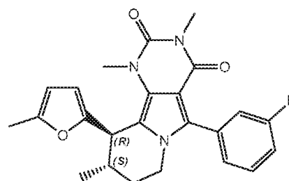
(9 S ,10 R )-5-(3-fluorophenyl)-1,3,9-trimethyl-10-(5-methylfuran-2-yl)-7,8,9,10-tetrahydropyrimido[4,5- a ]indolizine-2,4(1 H ,3 H )-dione
