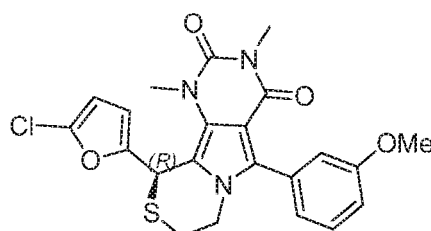
(R)-10-(5-chlorofuran-2-yl)-5-(3-methoxyphenyl)-1,3-dimethyl-7,8-dihydro-1H-pyrimido[4',5':3,4]pyrrolo[2,1-c][1,4]thiazine-2,4(3H,10H)-dione
