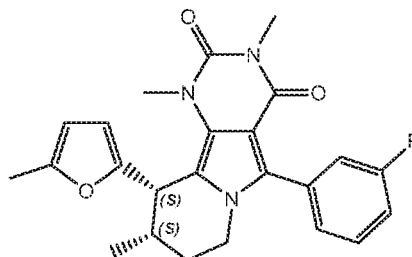
(9 S ,10 S )-5-(3-fluorophenyl)-1,3,9-trimethyl-10-(5-methylfuran-2-yl)-7,8,9,10-tetrahydropyrimido[4,5- a ]indolizine-2,4(1 H ,3 H )-dione
