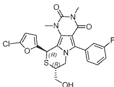
(8 R ,10 R )-10-(5-chlorofuran-2-yl)-5-(3-fluorophenyl)-8-(hydroxymethyl)-1,3-dimethyl-7,8-dihydro-1 H -pyrimido[4',5':3,4]pyrrolo[2,1- c ][1,4]thiazine-2,4(3 H ,10 H )-dione
