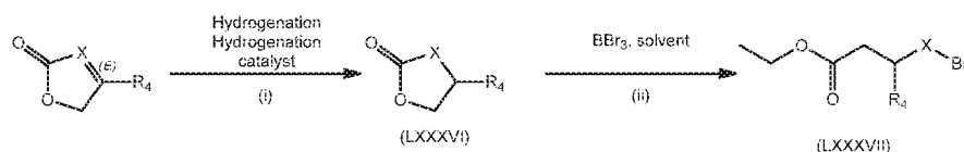
Scheme 23
