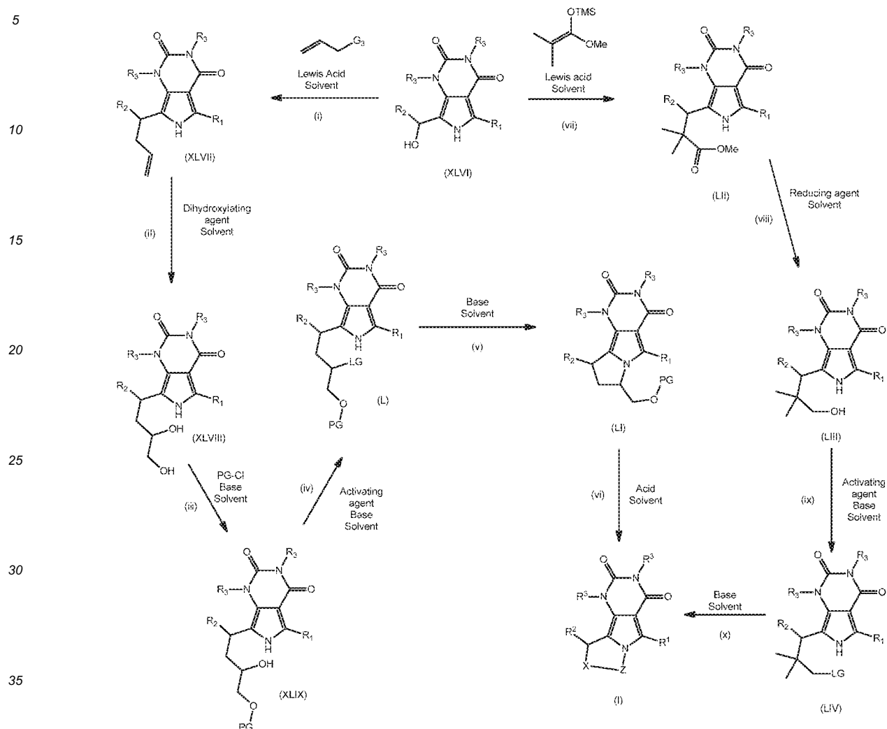
Scheme 14
