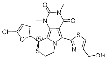
(R)-10-(5-chlorofuran-2-yl)-5-(4-(hydroxymethyl)thiazol-2-yl)-1,3-dimethyl-7,8-dihydro-1H-pyrimido[4',5':3,4]pyrrolo[2,1-c][1,4]thiazine-2,4(3H,10H)-dione
