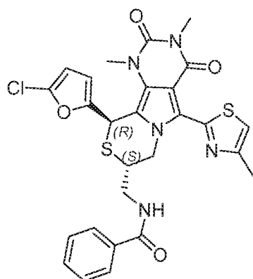
N-(((8S,10R)-10-(5-chlorofuran-2-yl)-1,3-dimethyl-5-(4-methylthiazol-2-yl)-2,4-dioxo-2,3,4,7,8,10-hexahydro-1H-pyrimido[4',5':3,4]pyrrolo[2,1-c][1,4]thiazin-8-yl)methyl)benzamide
