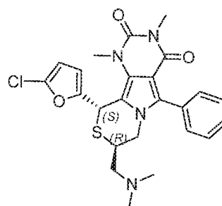
(8 R ,10 S )-10-(5-chlorofuran-2-yl)-8-((dimethylamino)methyl)-1,3-dimethyl-5-phenyl-7,8-dihydro-1 H -pyrimido[4',5':3,4]pyrrolo[2,1-c][1,4]thiazine-2,4(3 H ,10 H )-dione
