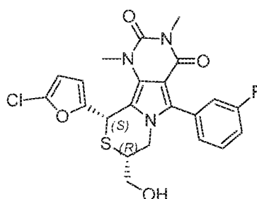
(8 R ,10 S )-10-(5-chlorofuran-2-yl)-5-(3-fluorophenyl)-8-(hydroxymethyl)-1,3-dimethyl-7,8-dihydro-1 H -pyrimido[4',5':3,4]pyrrolo[2,1- c ][1,4]thiazine-2,4(3 H ,10 H )-dione
