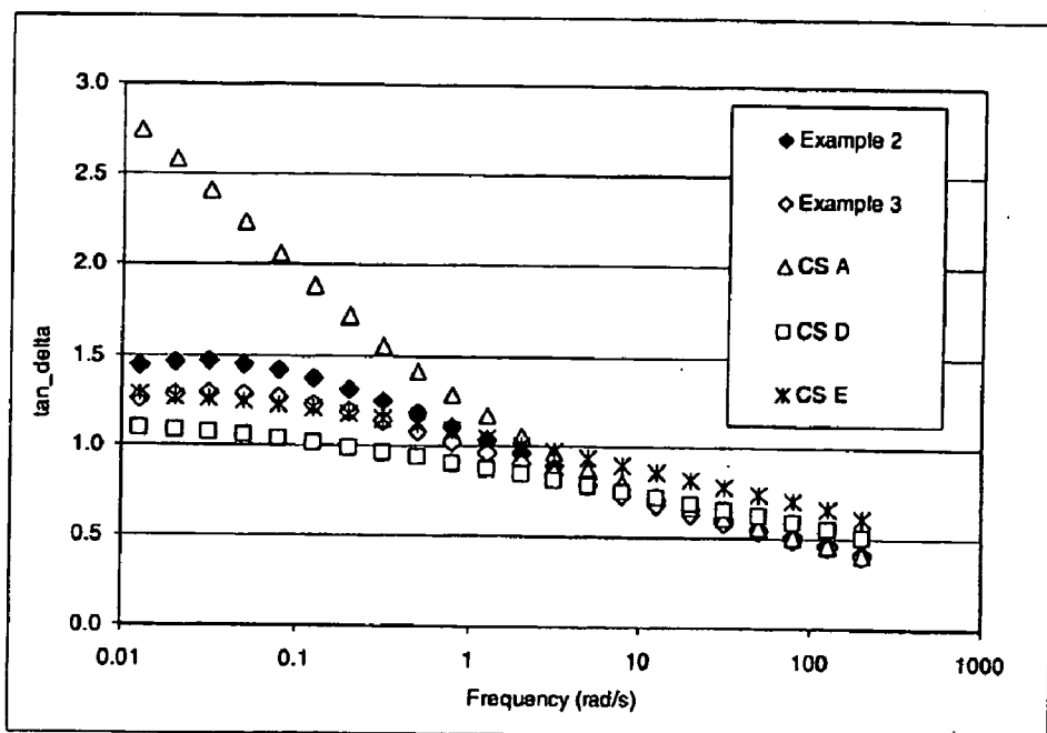
FIG. 3 Tan Delta Comparison
