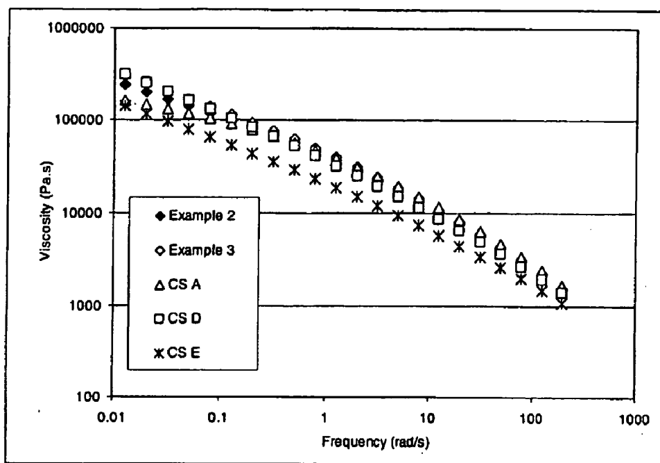
FIG. 2 Low Shear Viscosity Comparison
