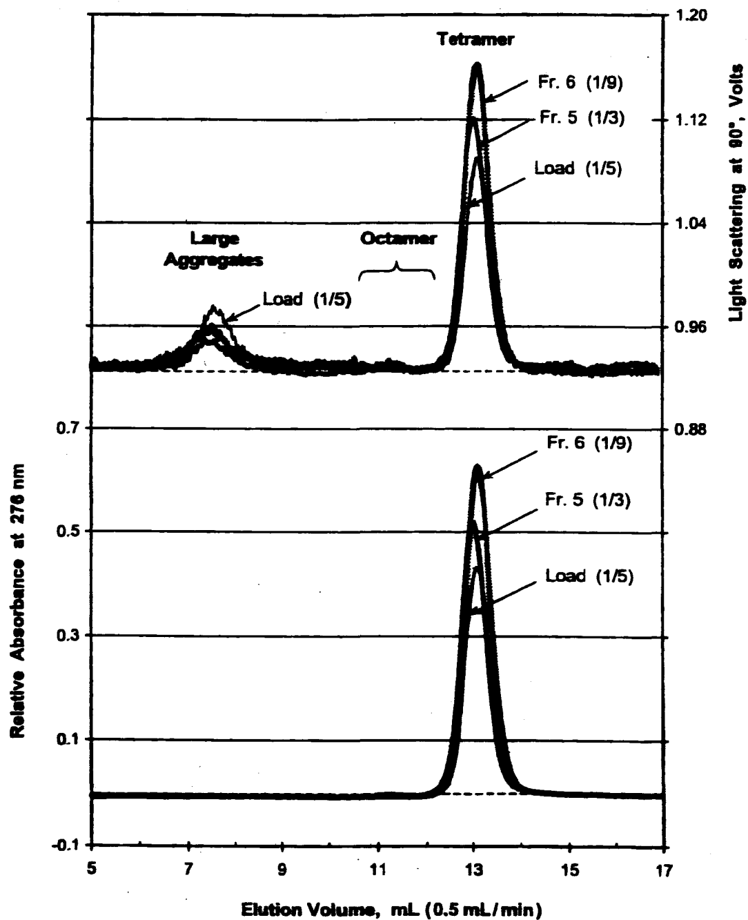
Size-Exclusion HPLC on Superdex 200 of Unfractionated PKS Uricase (Load) and Mono Q Column Fractions in the Low-Salt Pool
