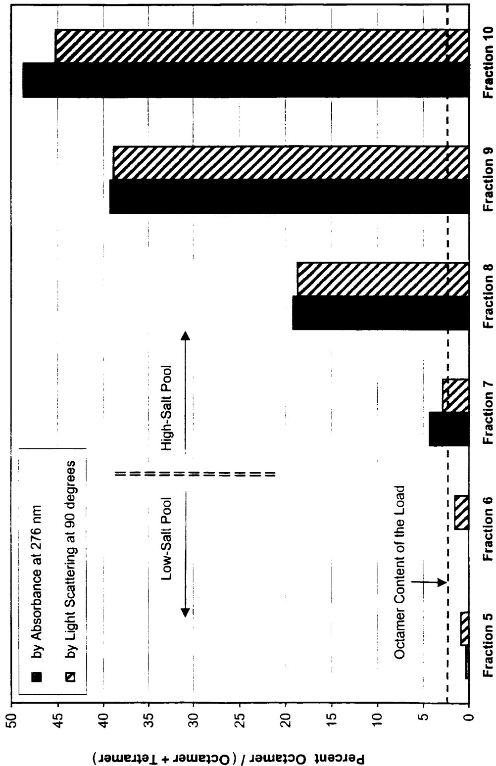
Octamer Content of Mono Q Column Fractions of PKS Urlicase
