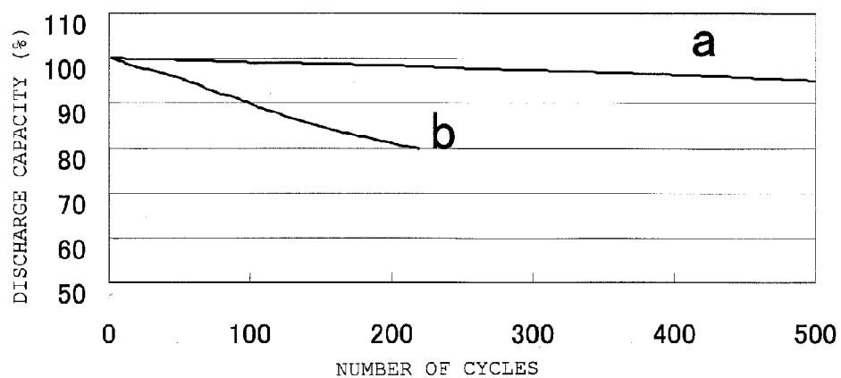
FIG. 1 CYCLE TEST AT 25°C
