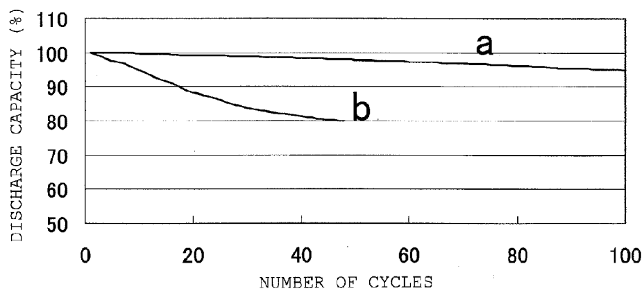
FIG. 2 CYCLE TEST AT 60°C
