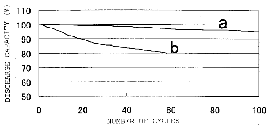
FIG. 3 CYCLE TEST AT -10^{\circ}\text{C}
