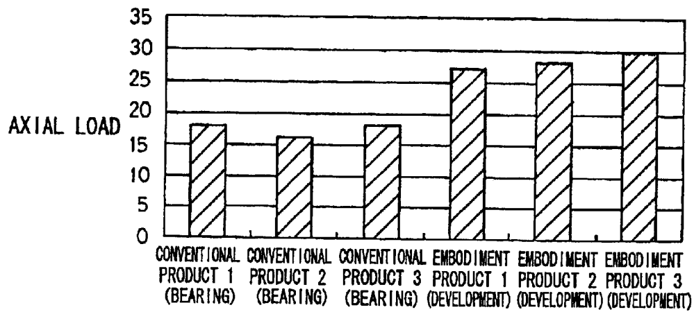
SMALL AMOUNT OF OIL SUPPLY SEIZURE TEST
