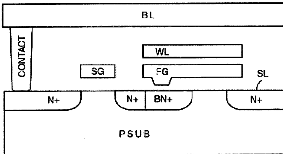
FIG. 1C (Prior Art)
