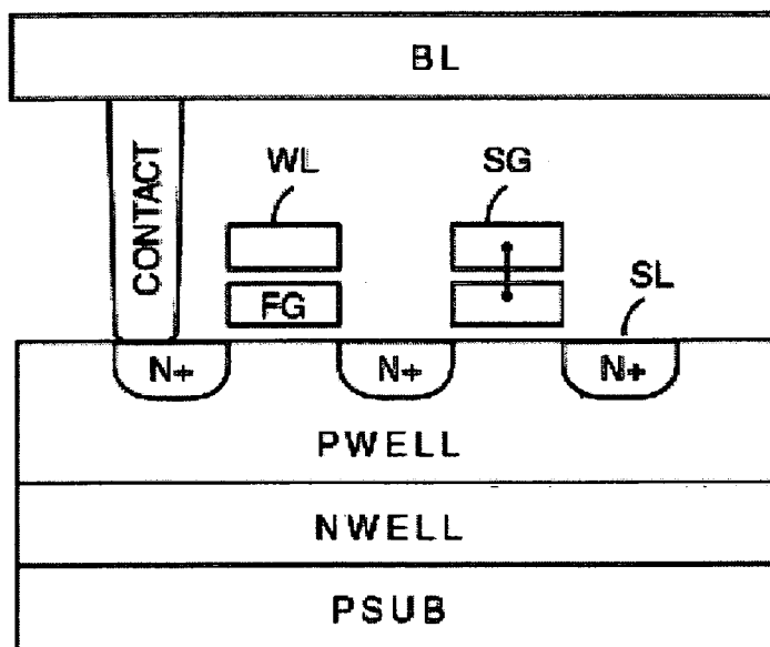
FIG. 4C (Prior Art)
