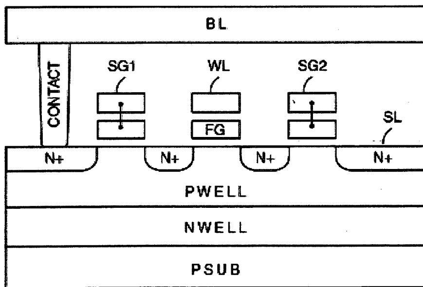
FIG. 2C (Prior Art)
