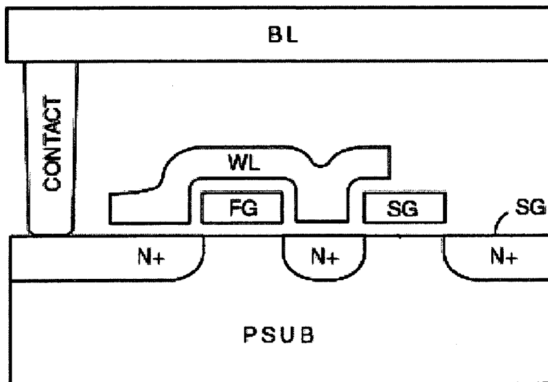
FIG. 5C (Prior Art)
