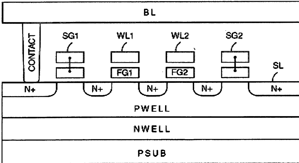
FIG. 3C (Prior Art)
