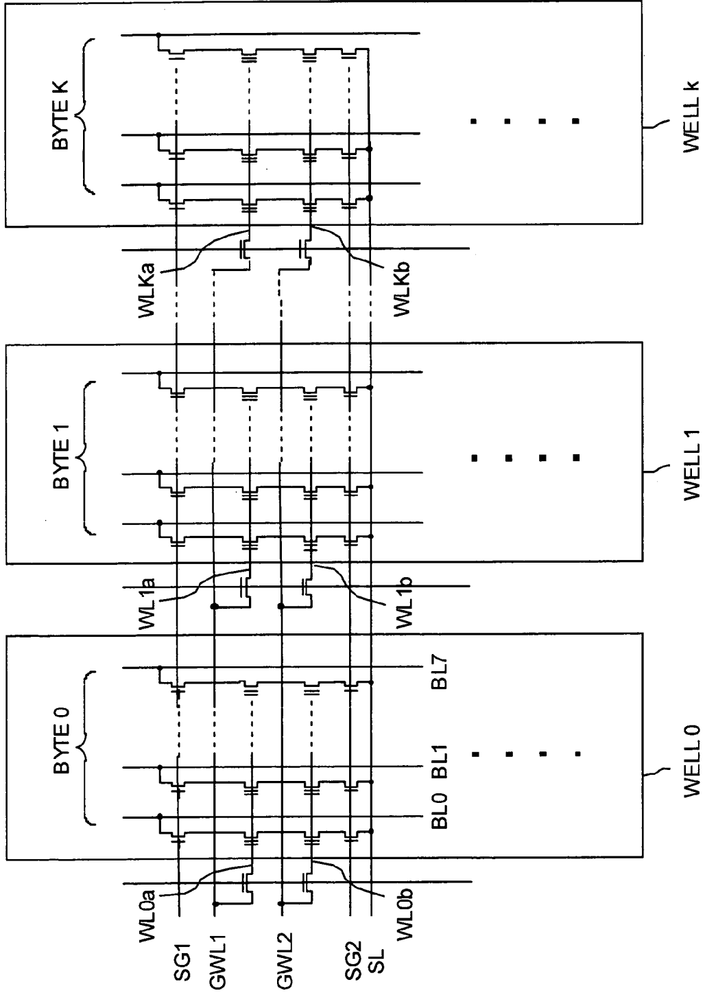
FIG. 15 (Prior Art)
