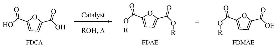
Scheme 1. Esterification of FDCA to FDMAE and FDAE
