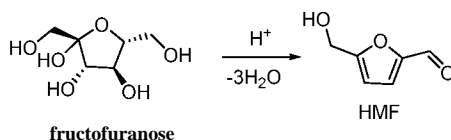
Scheme A. Catalytic dehydrative cyclization of fructose to HMF
