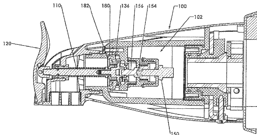
AUTO DIVERT CROSS-SECTION
