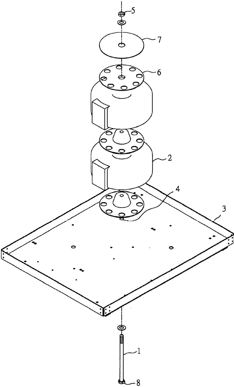
FIG. 1 PRIOR ART
