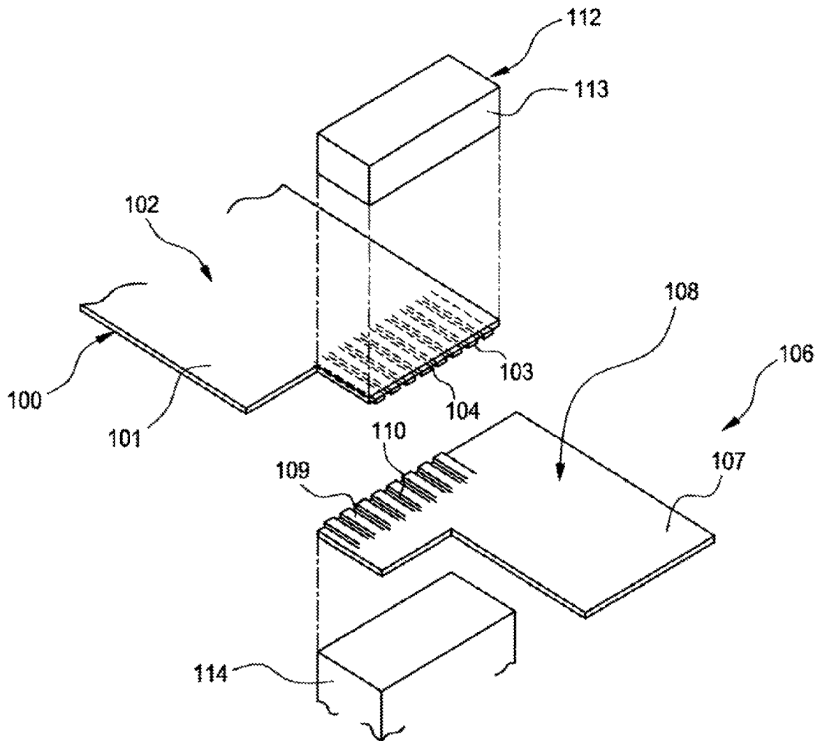
FIG. 9 PRIOR ART
