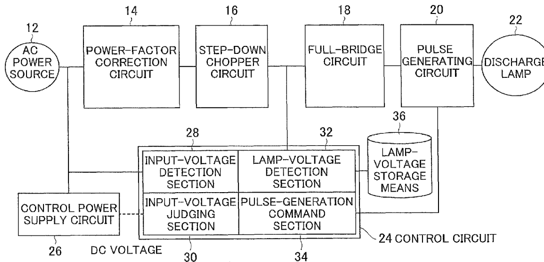
10 DISCHARGE LAMP LIGHTING DEVICE
