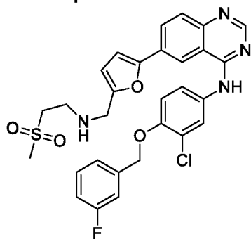
Lapatinib
