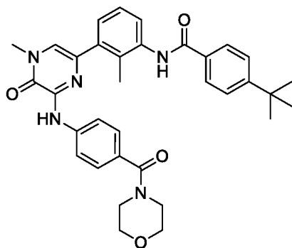
CGI-1746
