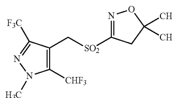
3-({[5-(difluoromethyl)-1-methyl-3-(trifluoromethyl)-1H-pyrazol-4-yl]methyl}sulfonyl)-5,5-dimethyl-4,5-dihydro-1,2-oxazole
