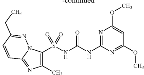
N-[(4,6-dimethoxypyrimidin-2-yl)carbamoyl]-6-ethyl-2-methylimidazo[1,2-b]pyridazine-3-sulfonamide
