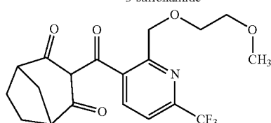
3-({2-[(2-methoxyethoxy)methyl]-6-(trifluoromethyl)pyridin-3-yl}carbonyl)bicyclo[3.2.1]octane-2,4-dione
