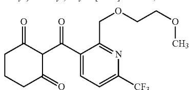
2-({2-[(2-methoxyethoxy)methyl]-6-(trifluoromethyl)pyridin-3-yl}carbonyl)cyclohexane-1,3-dione
