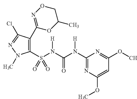
3-chloro-N-[(4,6-dimethoxypyrimidin-2-yl)carbamoyl]-1-methyl-4-(5-methyl-5,6-dihydro-1,4,2-dioxazin-3-yl)-1H-pyrazole-5-sulfonamide
