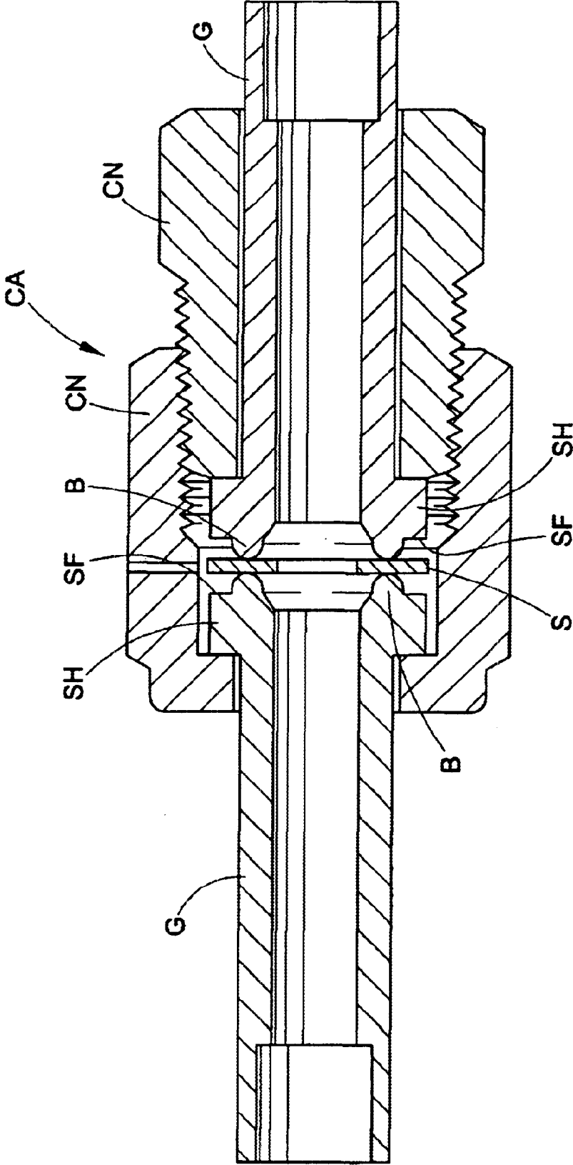
FIG. 1 (PRIOR ART)
