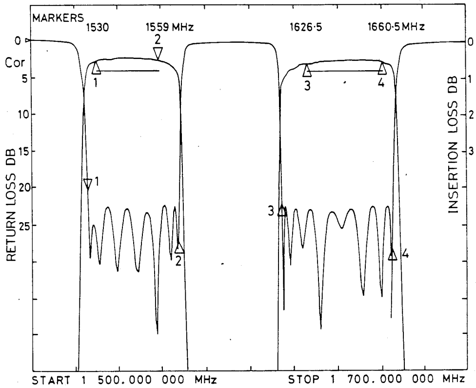
INSERTION LOSS AND RETURN LOSS
