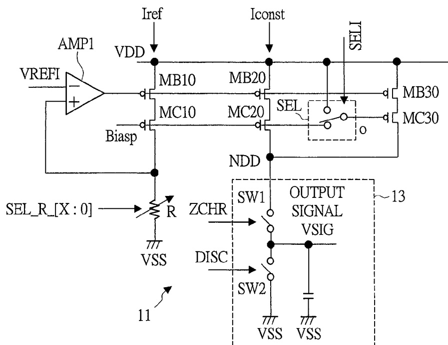
FREQUENCY-VOLTAGE CONVERTING CIRCUIT
