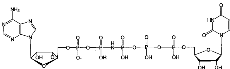
(c) AppNHpppU
