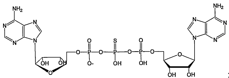
(b) A_{diol}ppCH_2ppA_{diol}
