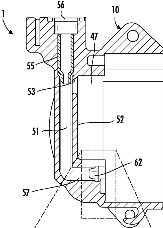
FIG. 2 PRIOR ART
