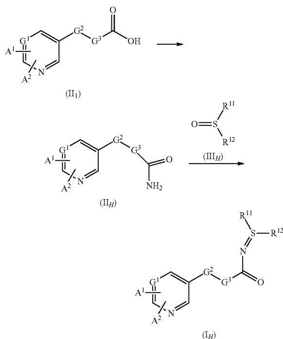
Reaction scheme 3
