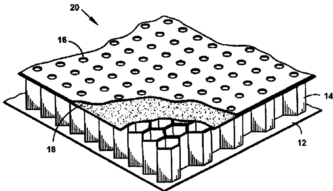
Fig. 2 (prior art)
