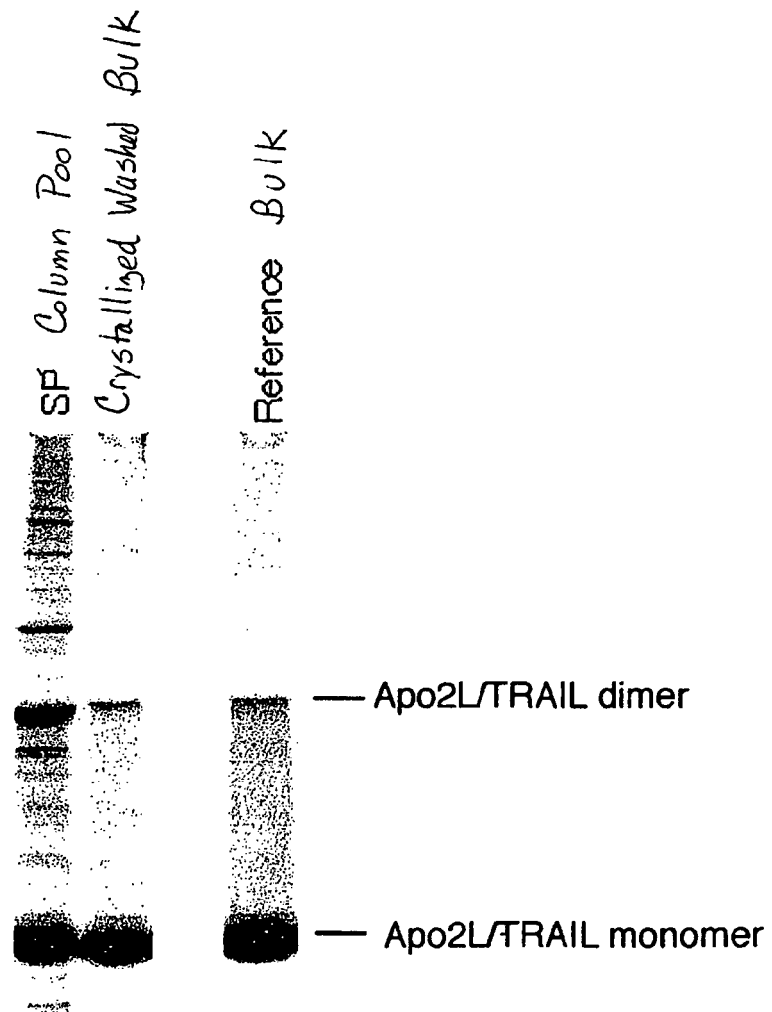
Figure 13 -SDS-PAGE silver stain purity of Apo2L/TRAIL purified by crystallization compared to a three-column step purified reference material.
