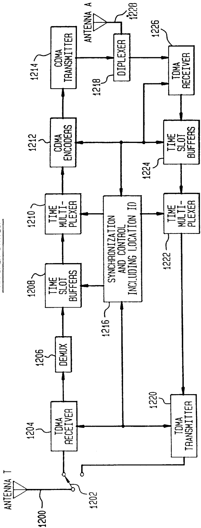
FIG. 12 TRANSFER STATION
