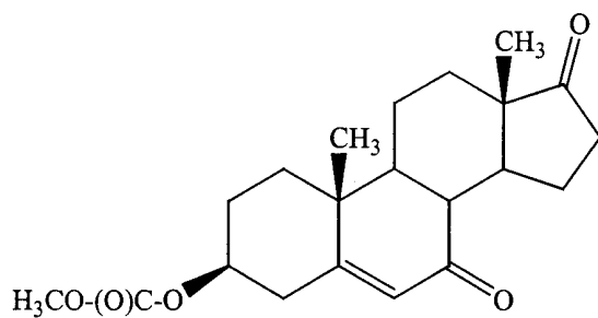
compound 10
