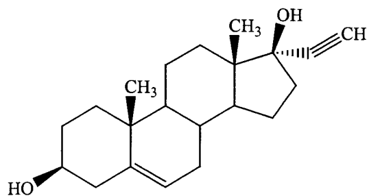
compound 6
