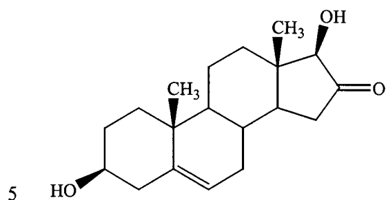
compound 8
