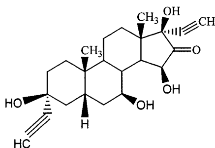
subgroup 13-1, compound 4.2.2.3,
