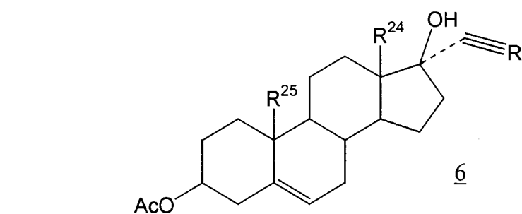
Scheme 6
