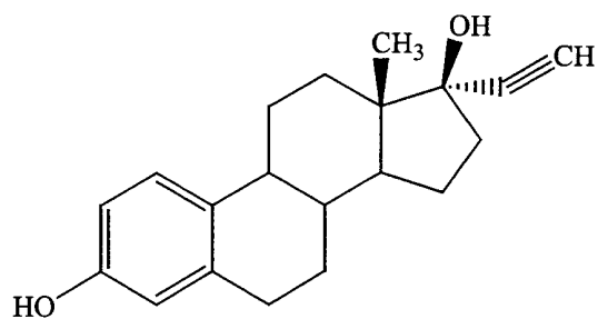
compound 4.
