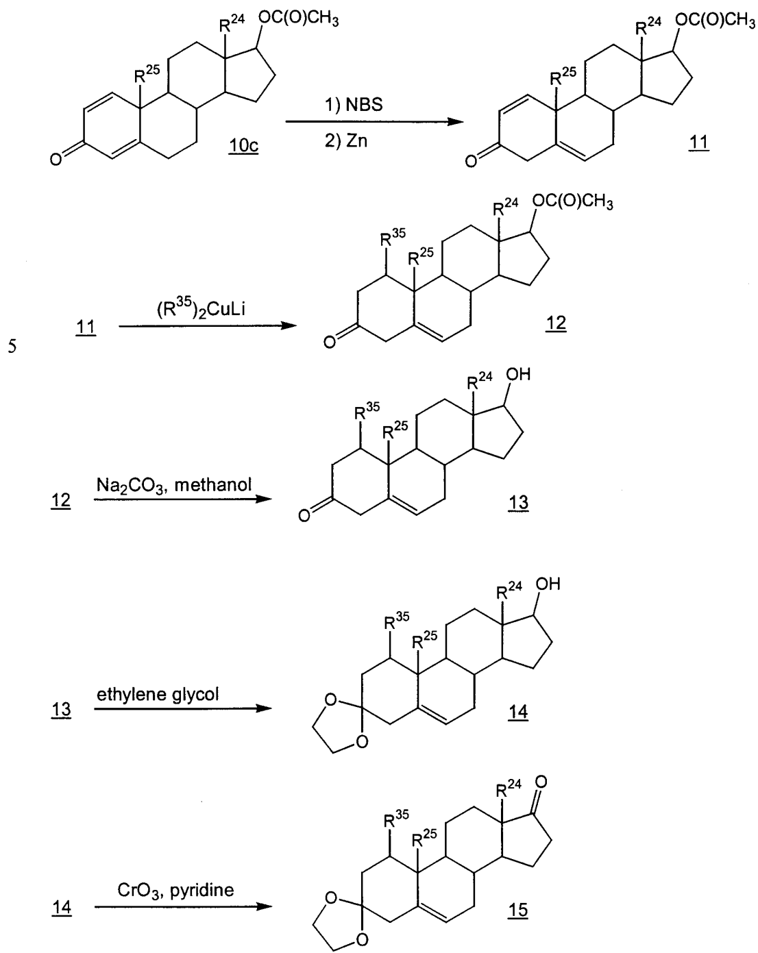
Scheme 11
