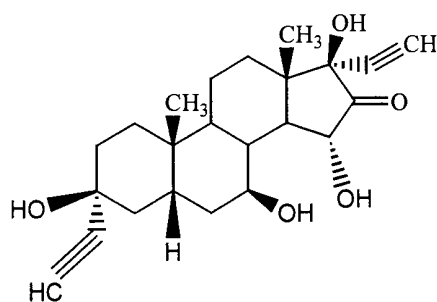
subgroup 13-2, compound 4.2.2.3.
