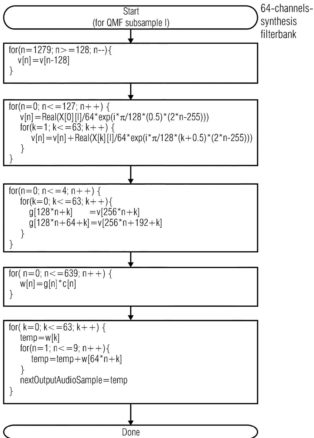
FIG 25C (CORRESPONDING TO FIG. 4.42 OF ISO/IEC 14496-3:2005(E))
