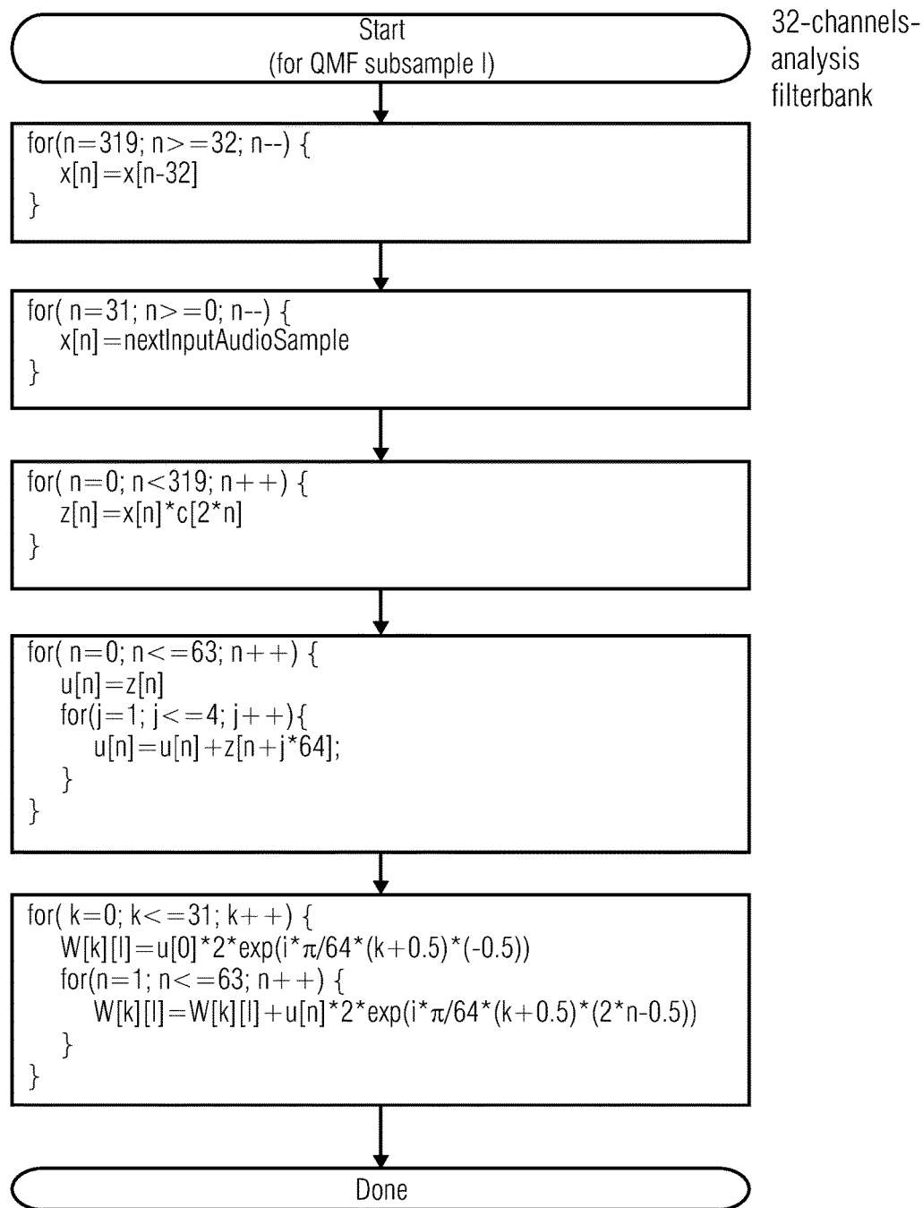
FIG 25B (CORRESPONDING TO FIG. 4.41 OF ISO/IEC 14496-3:2005(E))
