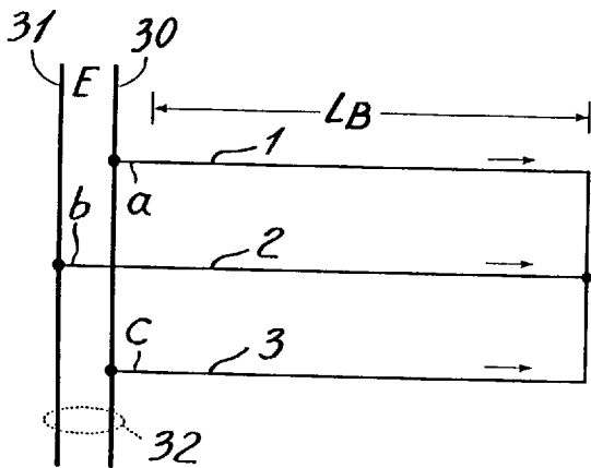
SINGLE-PHASE FEEDER FIG. 13a
