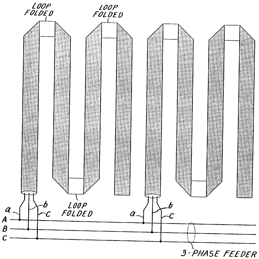
FIG. 10 Three-phase similar-flow configuration
