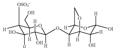
Formula 2-kappa-carrabiose unit
