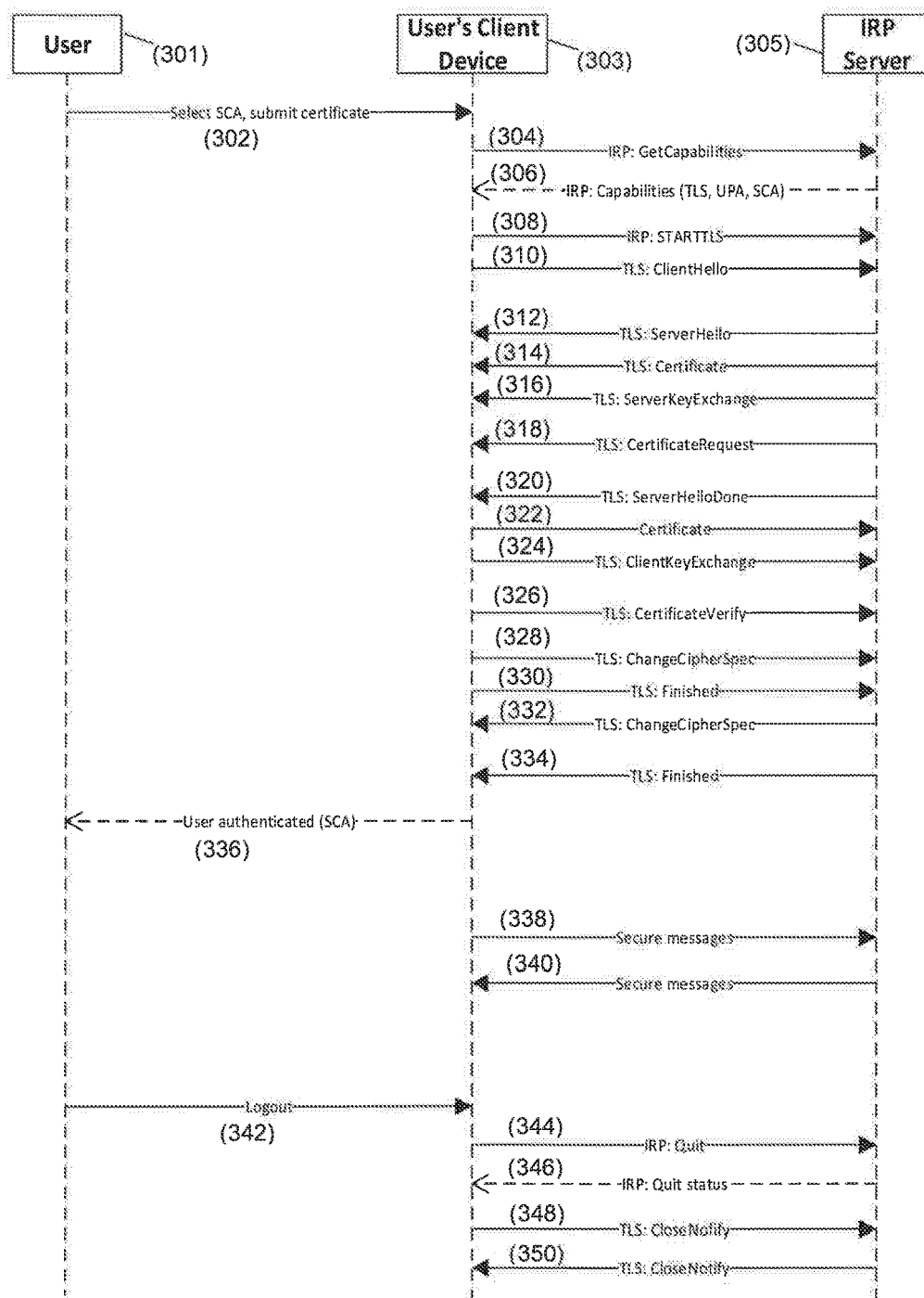
SCA – TLS 1.2 with Mutual Authentication
