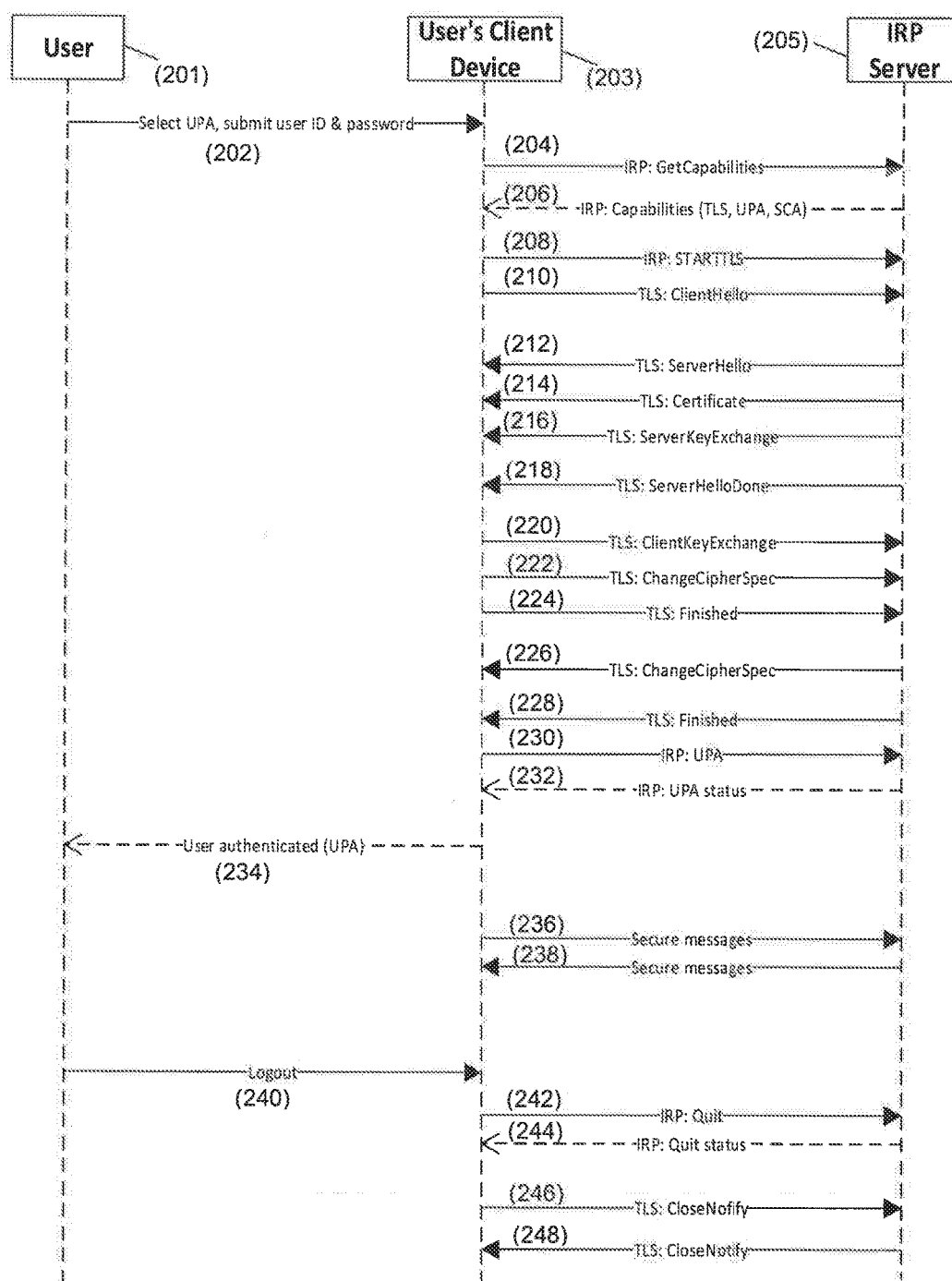
UPA – TLS 1.2 with Server Authentication & Password Authentication
