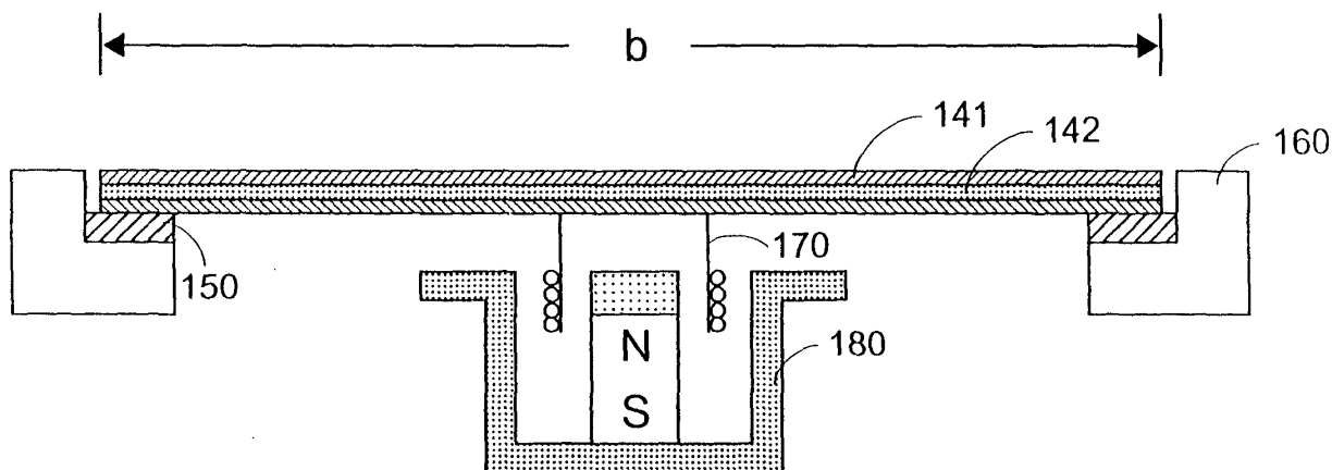
A-A Cross section
