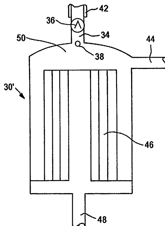
FIG. 4 PRIOR ART
