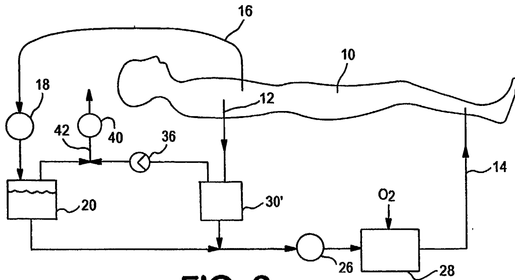
FIG. 3 PRIOR ART
