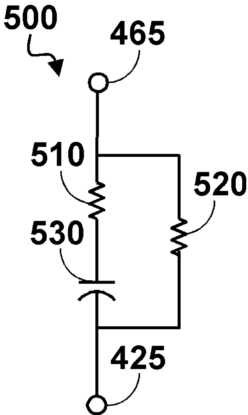
Fig. 5 (Prior Art)
