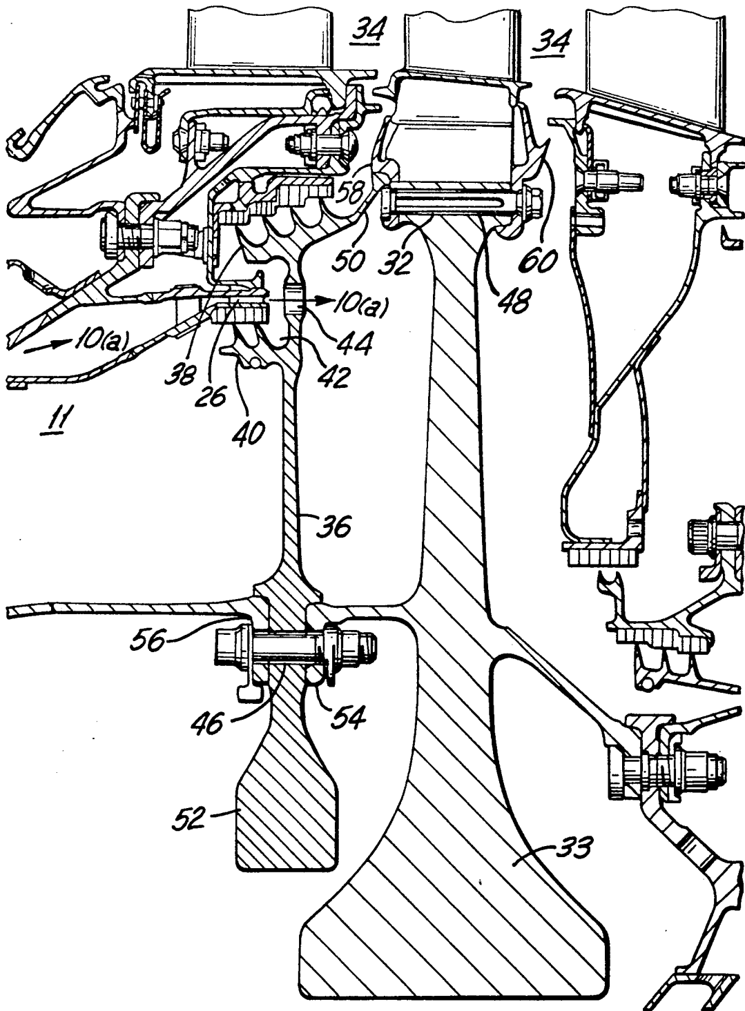
FIG. 2 (PRIOR ART)
