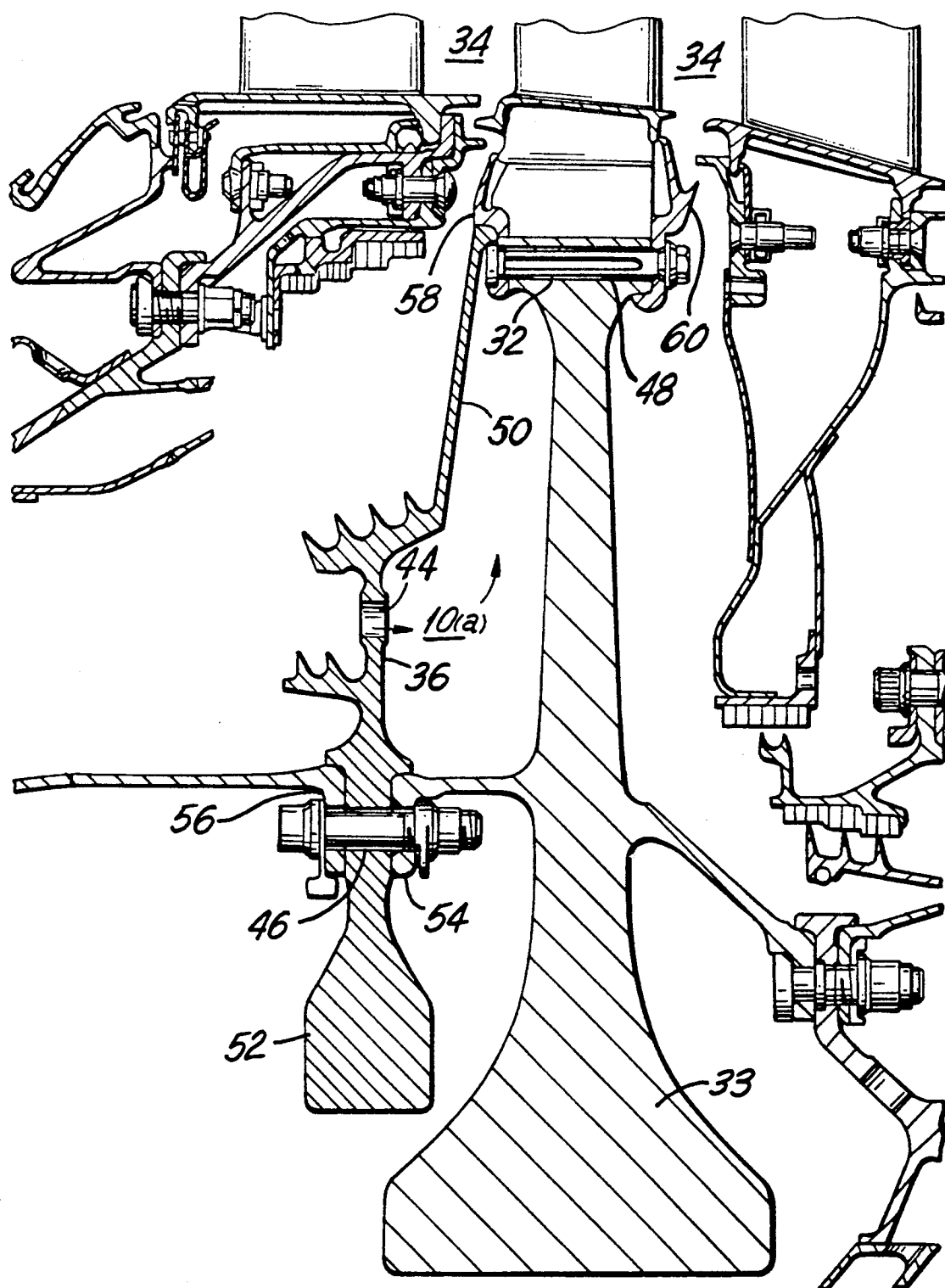
FIG.3 (PRIOR ART)
