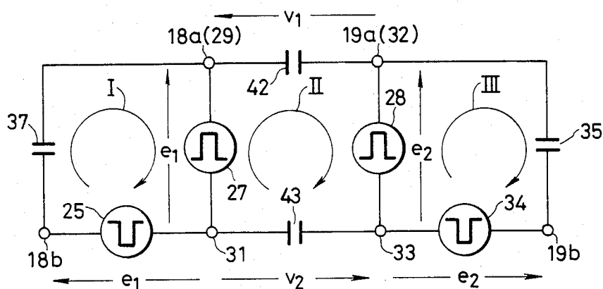
FIG. 4 PRIOR ART
