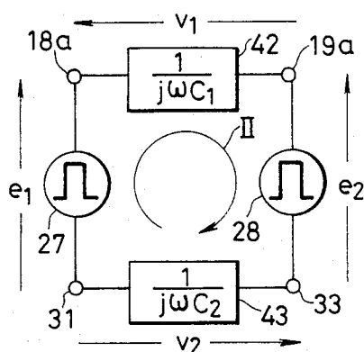
FIG. 5 PRIOR ART
