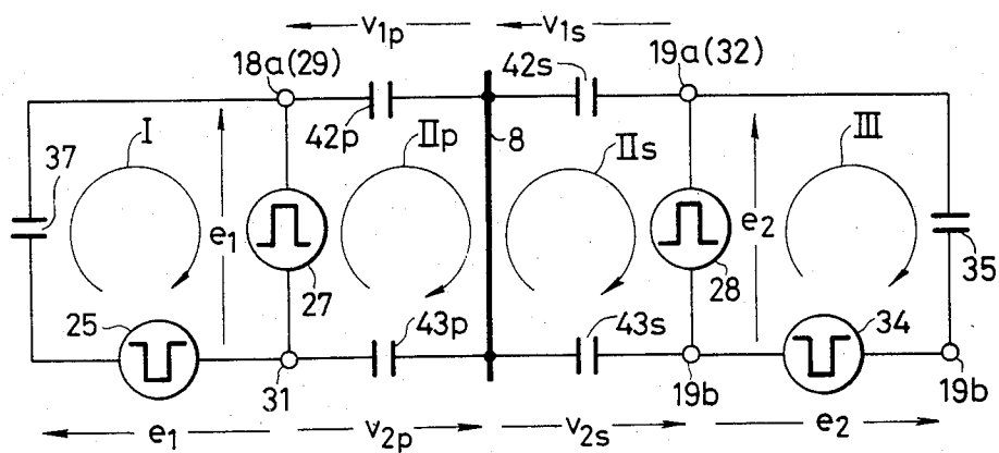
FIG. 7 PRIOR ART
