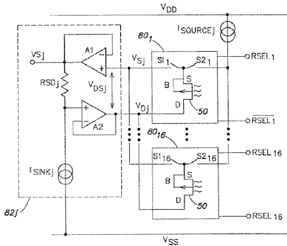
85] FIG. 3 (Prior Art)
