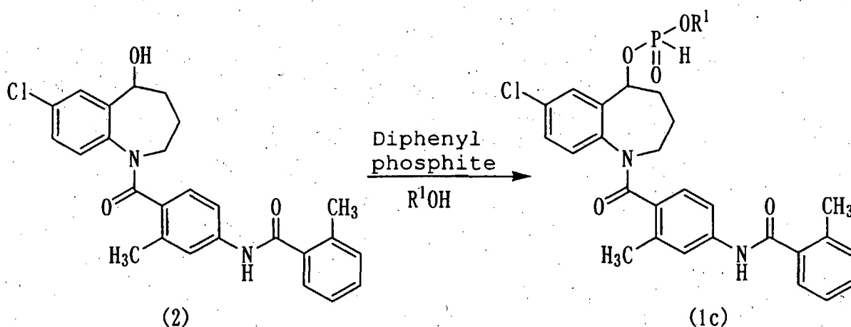
Reaction scheme-3
