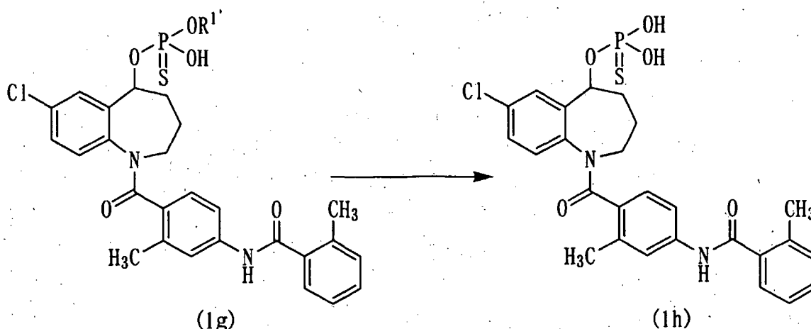
Reaction scheme-7
