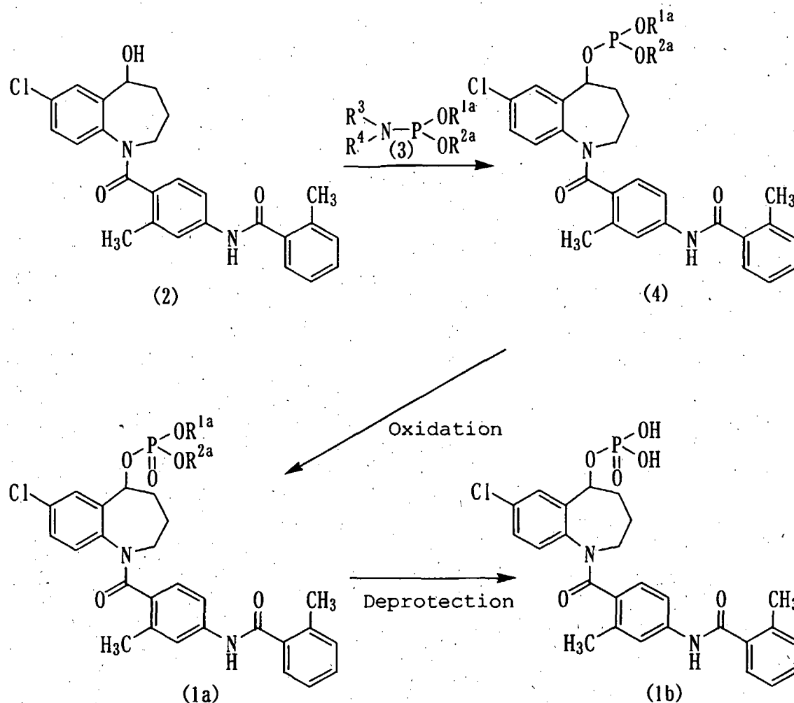
Reaction scheme-1
