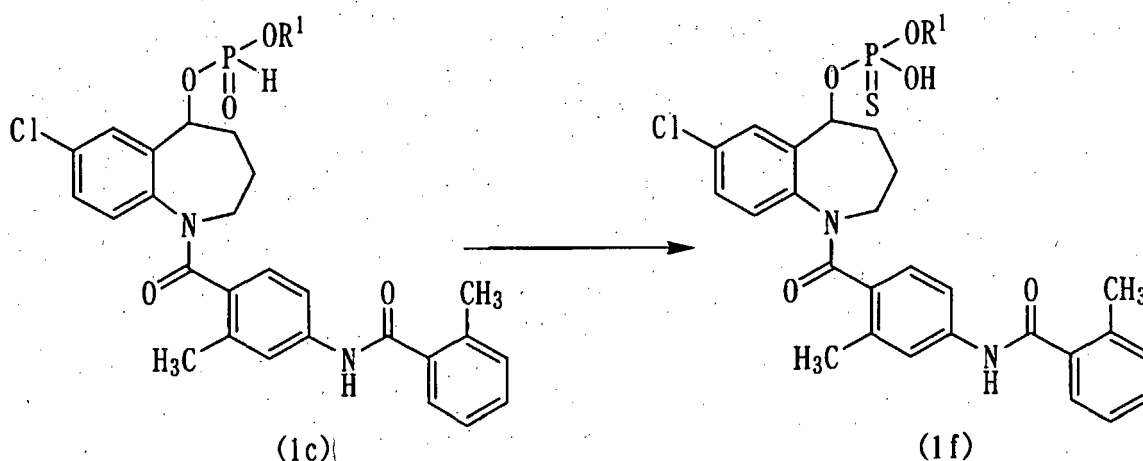
Reaction scheme-6
