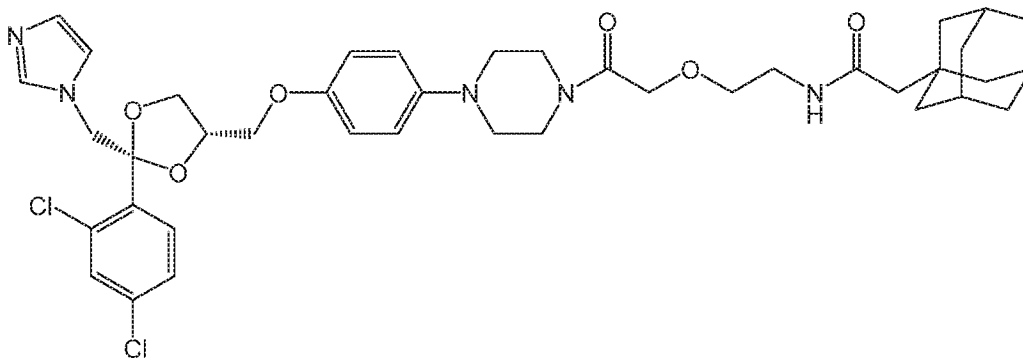
Compound 41
