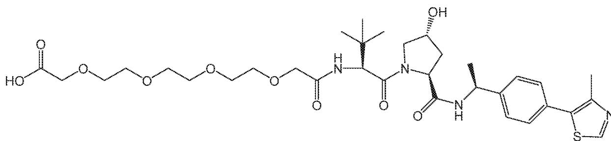
Compound 36
