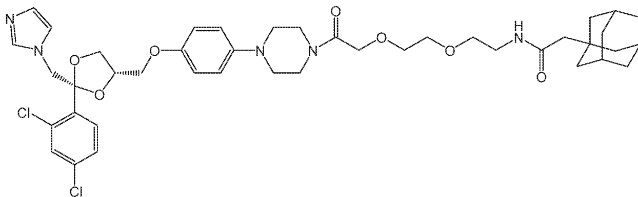
Compound 42
