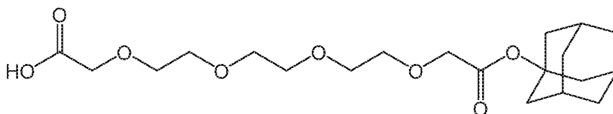
Compound 28
