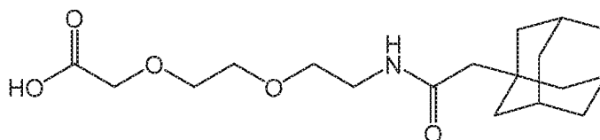
Compound 7
