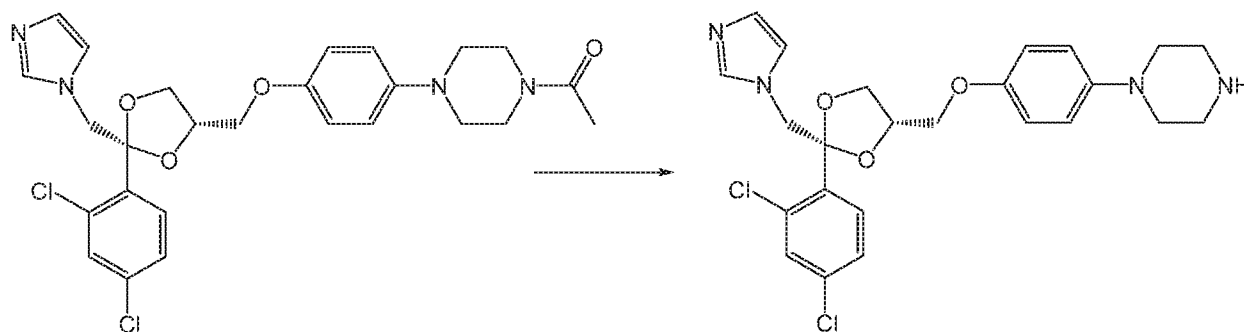
Scheme 13
