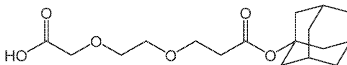
Compound 23
