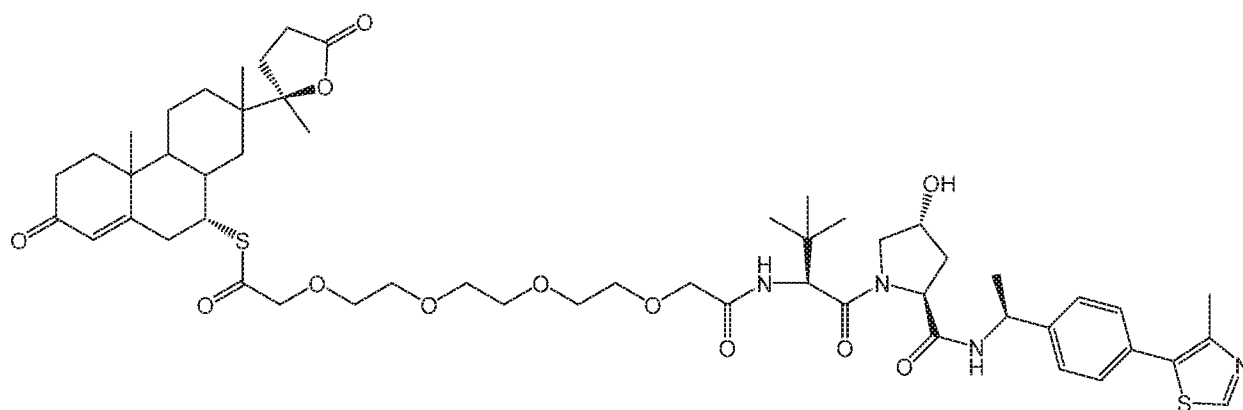
Compound 46
