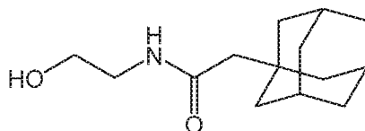
Compound 1
