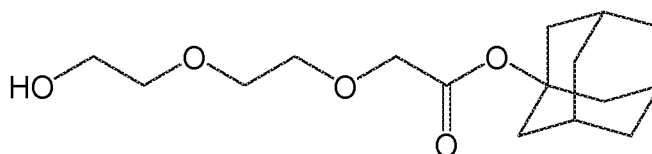
Compound 31
