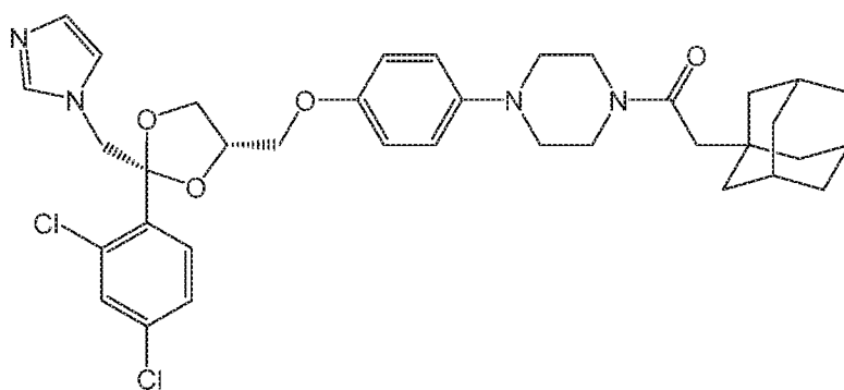
Compound 40
