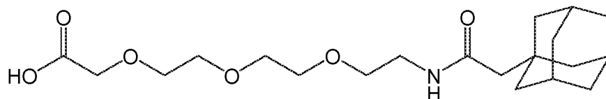
Compound 8
