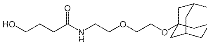
Compound 18
