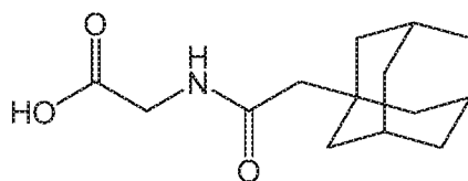
Compound 5
