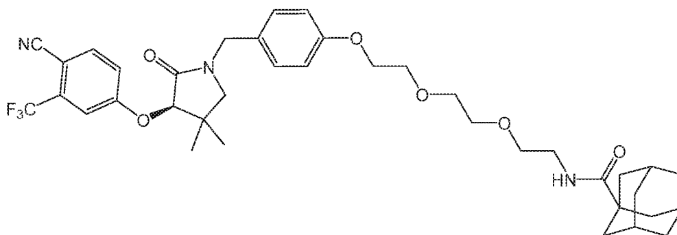
Compound 52
