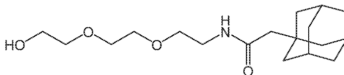
Compound 3
