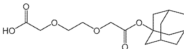
Compound 26
