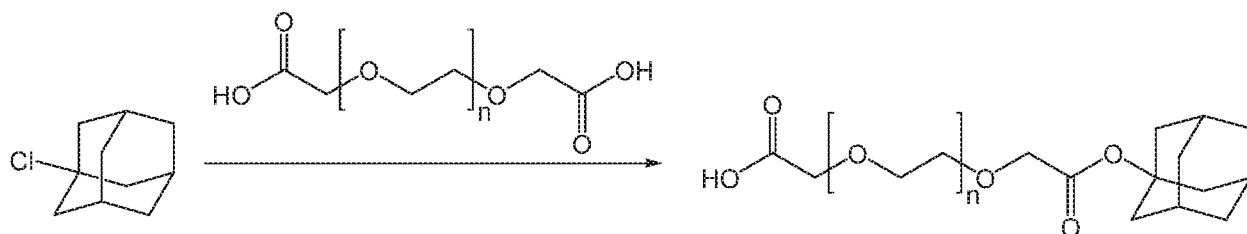
Scheme 9
