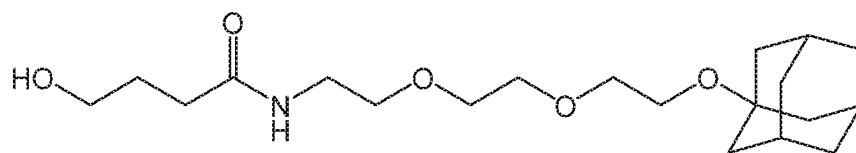
Compound 19
