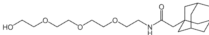
Compound 4
