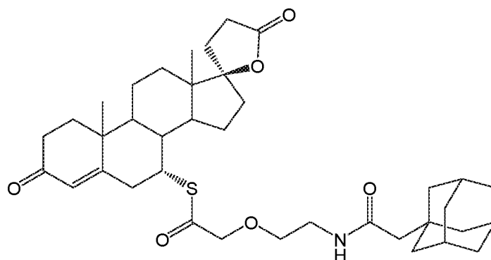
Compound 38
