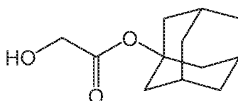
Compound 29
