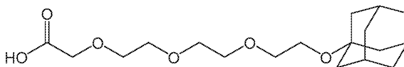
Compound 16
