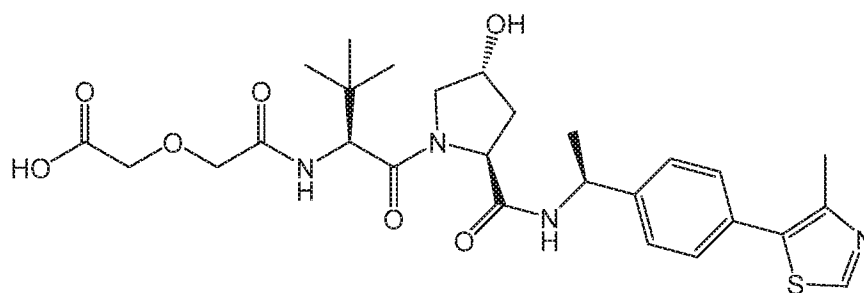
Compound 33
