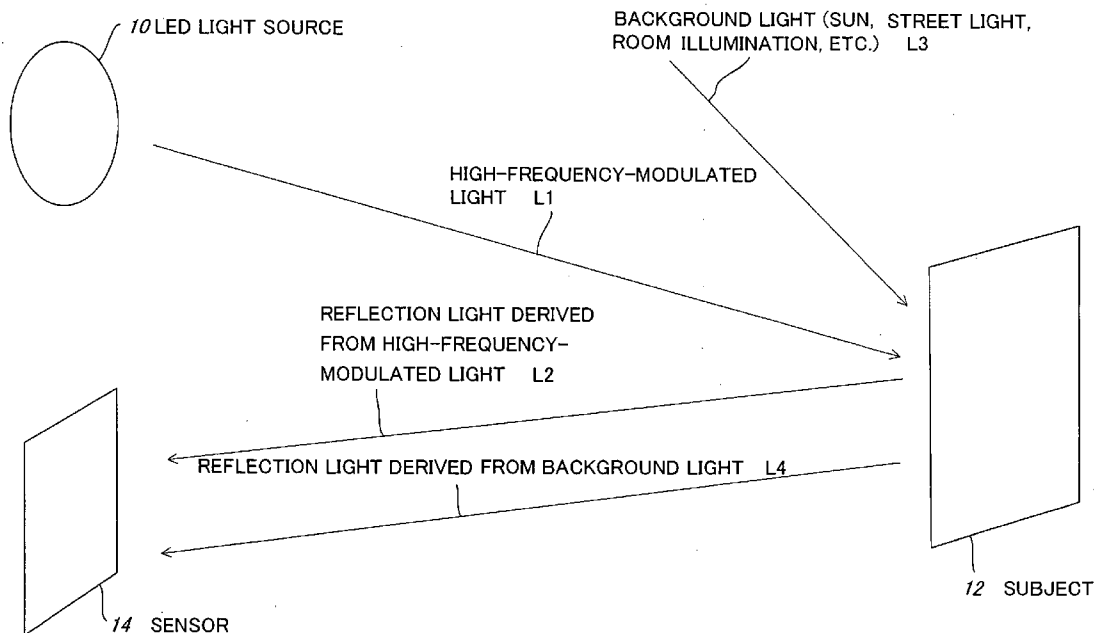
OUTLINE OF TIME-OF-FLIGHT MEASUREMENT METHOD
