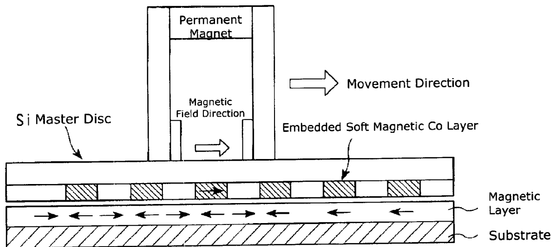
Transfer Pattern Writing Step
