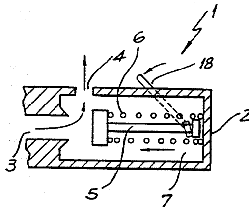
FIG. 2 PRIOR ART
