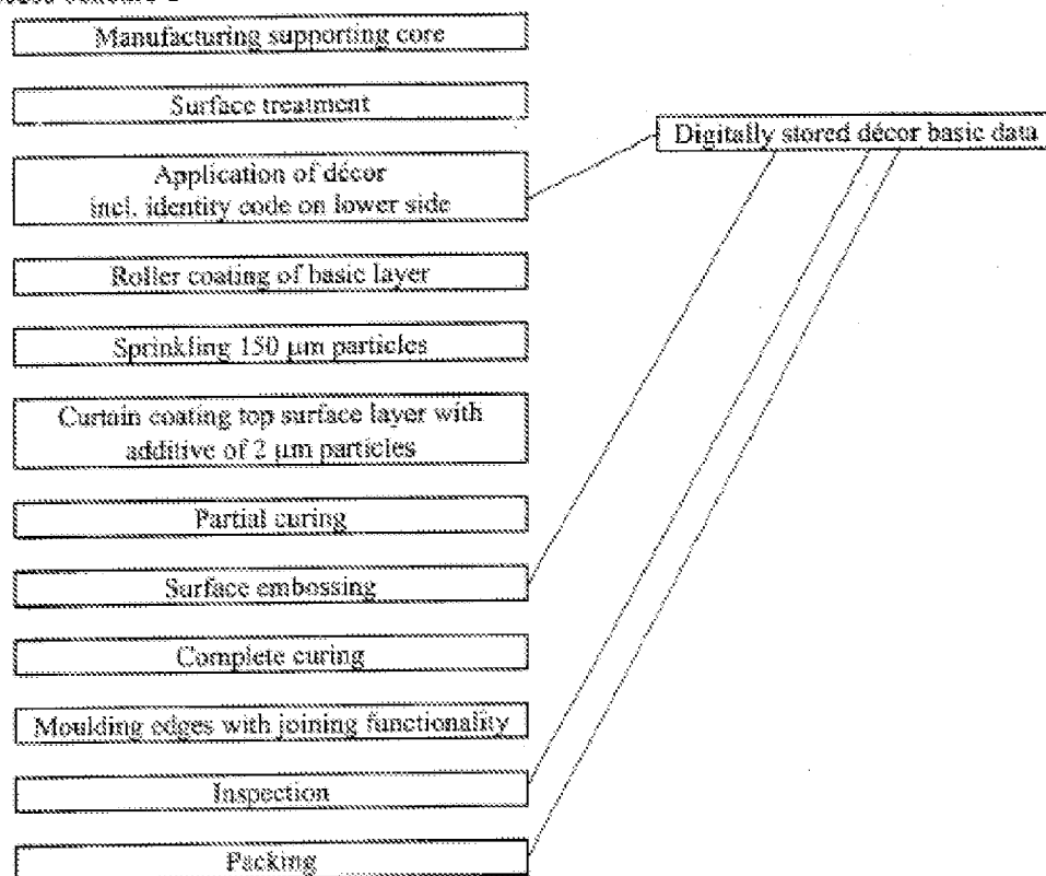
Process scheme 2
