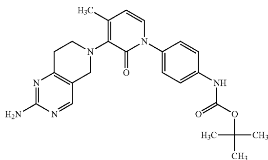
tert-butyl {4-[3-(2-amino-7,8-dihydropyrido[4,3-d]pyrimidin-6(5H)-yl)-4-methyl-2-oxopyridin-1(2H)-yl]phenyl}carbamate
