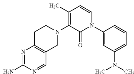
3-(2-amino-7,8-dihydropyrido[4,3-d]pyrimidin-6(5H)-yl)-1-[3-(dimethylamino)phenyl]-4-methylpyridin-2(1H)-one
