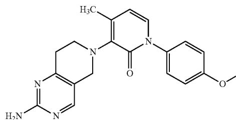
3-(2-amino-7,8-dihydropyrido[4,3-d]pyrimidin-6(5H)-yl)-1-(4-methoxyphenyl)-4-methylpyridin-2(1H)-one
