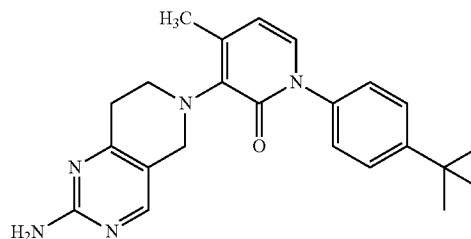
3-(2-amino-7,8-dihydropyrido[4,3-d]pyrimidin-6(5H)-yl)-1-(4-tert-butylphenyl)-4-methylpyridin-2(1H)-one
