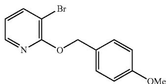
3-bromo-2-(4-methoxybenzyloxy)pyridine
