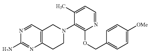
6-{2-[(4-methoxybenzyl)oxy]-4-methylpyridin-3-yl}-5,6,7,8-tetrahydropyrido[4,3-d]pyrimidin-2-amine
