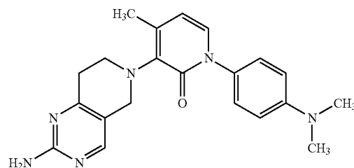
3-(2-amino-7,8-dihydropyrido[4,3-d]pyrimidin-6(5H)-yl)-1-[4-(dimethylamino)phenyl]-4-methylpyridin-2(1H)-one
