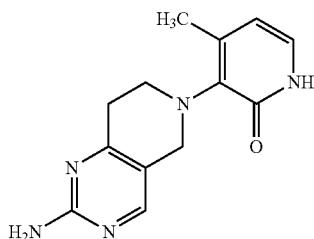
3-(2-amino-7,8-dihydropyrido[4,3-d]pyrimidin-6(5H)-yl)-4-methylpyridin-2(1H)-one
