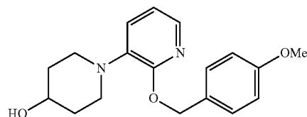
2'-(4-Methoxybenzyloxy)-3,4,5,6-tetrahydro-2H-[1,3']bipyridinyl-4-ol
