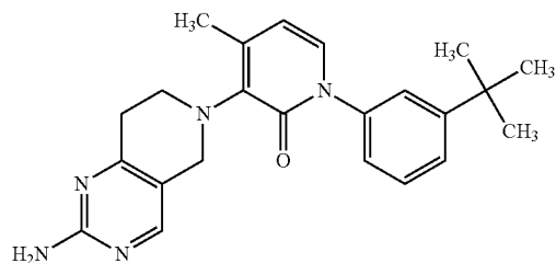
3-(2-amino-7,8-dihydropyrido[4,3-d]pyrimidin-6(5H)-yl)-1-(3-tert-butylphenyl)-4-methylpyridin-2(1H)-one
