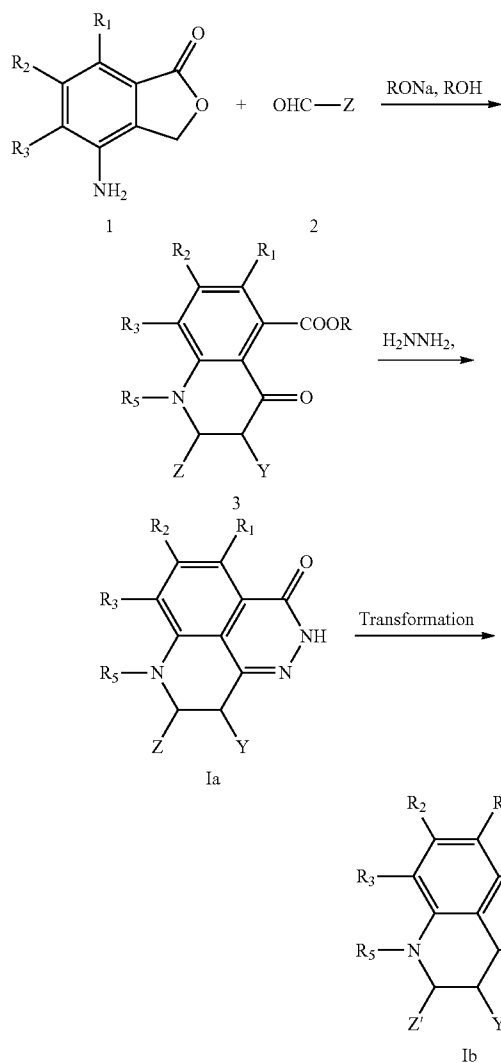
Synthetic Scheme 1
