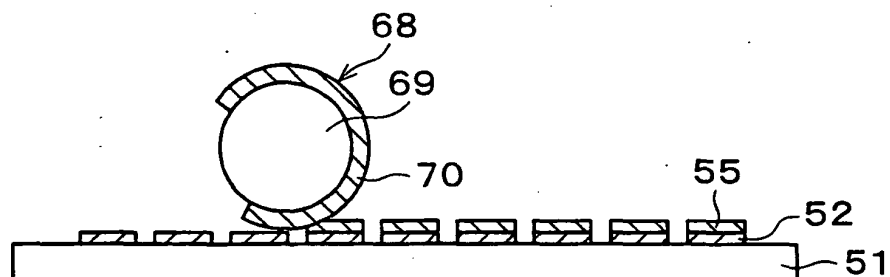
FIG. 12 (b) FORMATION OF HOLE TRANSPORT LAYER
