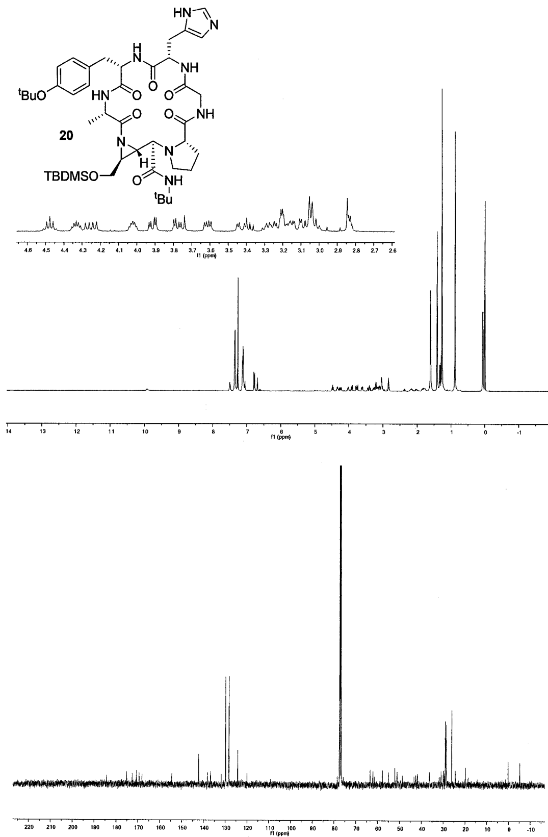
Figure 24. ^1\text{H} and ^{13}\text{C} NMR spectra for cyclic product 20.
