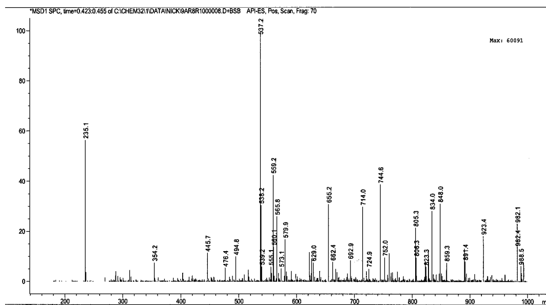
Figure 28. Crude LC-MS(ESI) analysis of HATU-mediated cyclization of Pro-Gly-Gly-Gly at 0.2M
