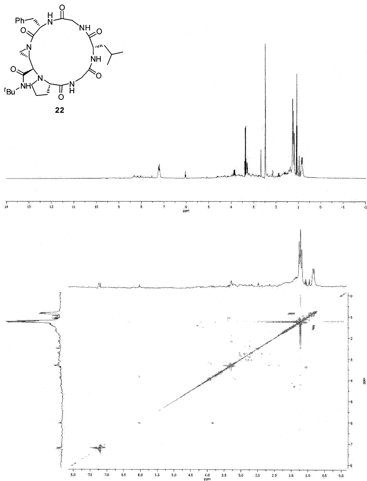
Figure 26. ^1\text{H} and COSY NMR spectra for cyclic product 22.
