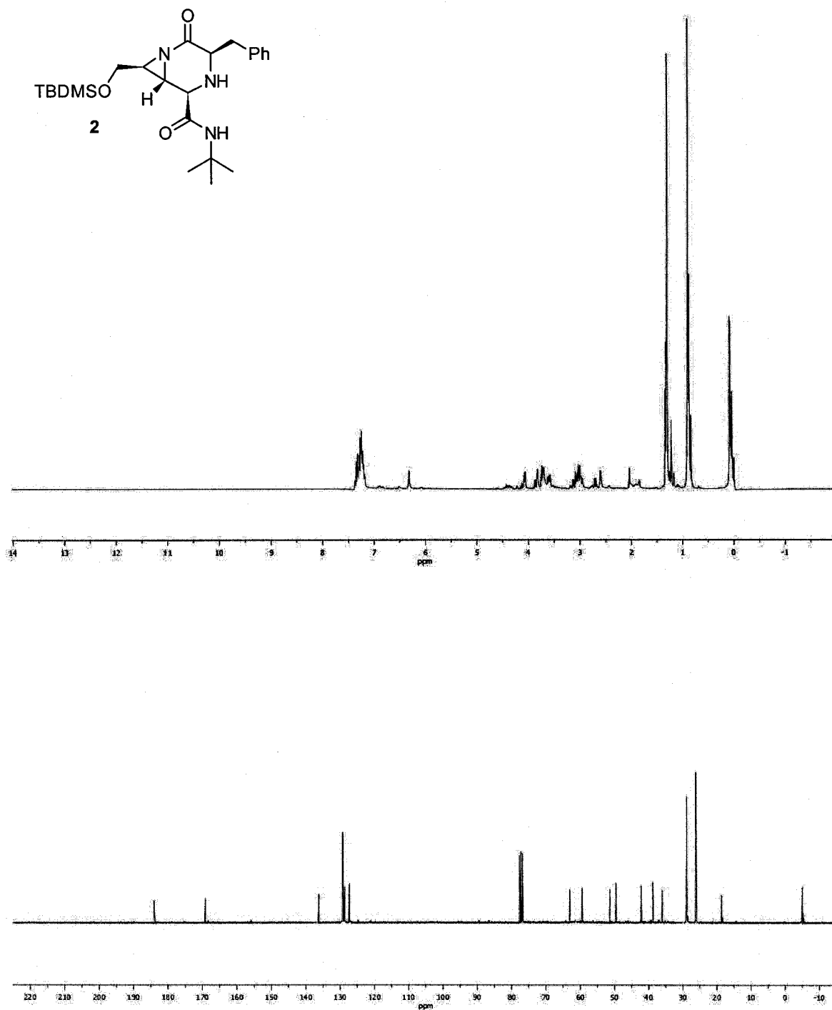
Figure 6. 1 H and 13 C NMR spectra for cyclic product 2.
