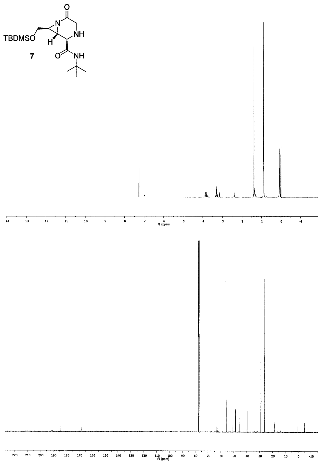
Figure 11. 1 H and 13 C NMR spectra for cyclic product 7.
