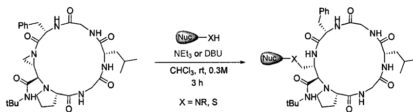
Figure 30. Nucleophilic ring-opening of aziridine-containing cyclic peptides.
