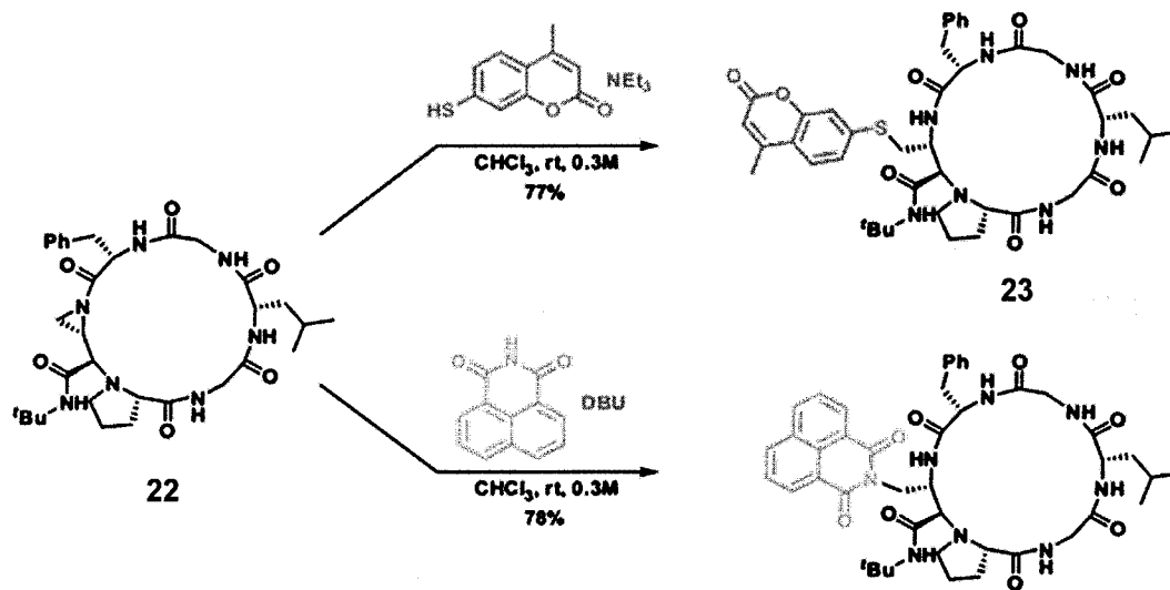
Scheme 3. Late-stage, site-specific attachment of fluorescent tags to a cyclic peptide.
