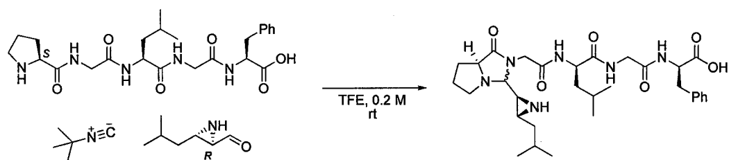
Figure 2. Mismatched reaction leads only to amination products.
