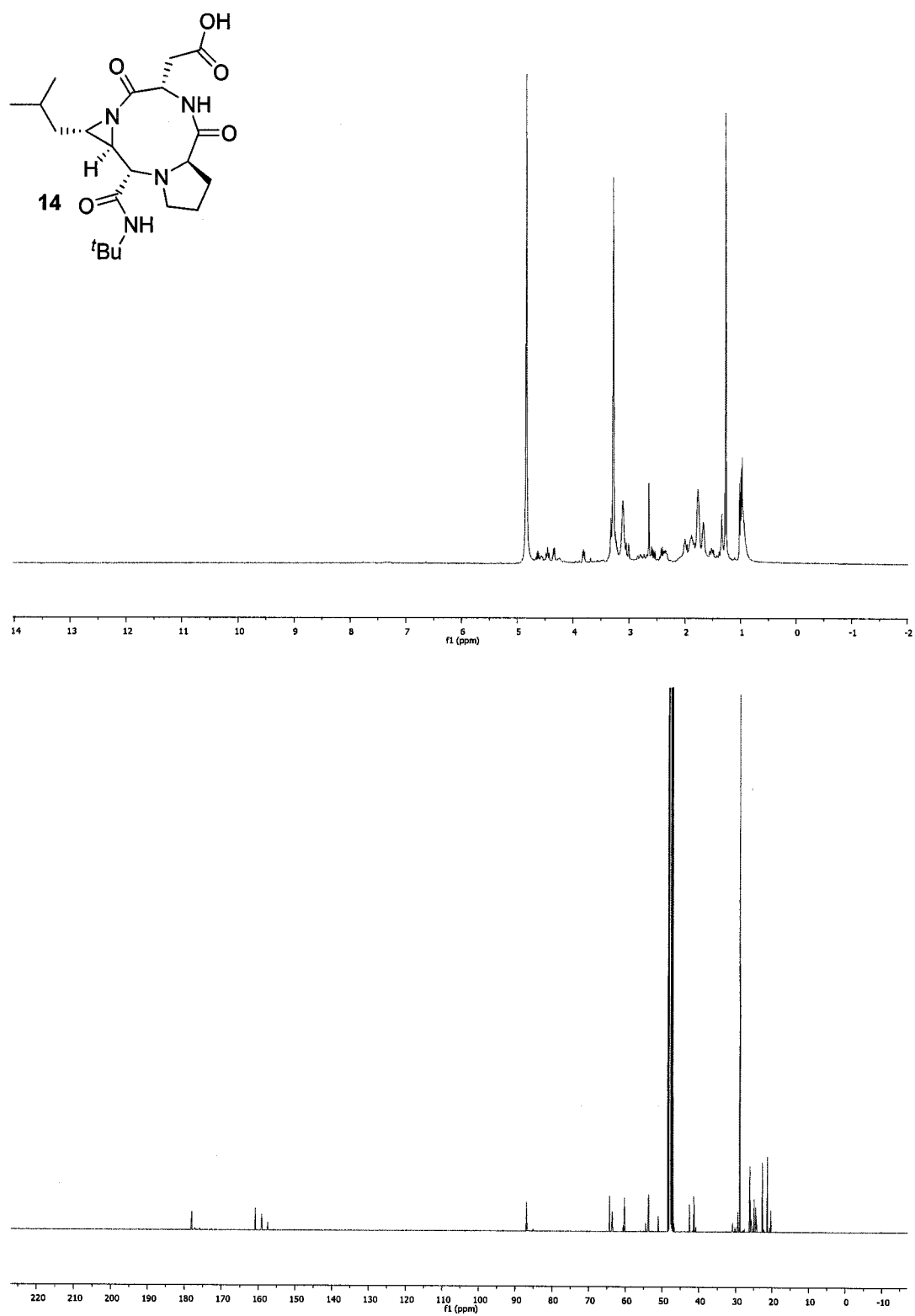
Figure 18. ^1\text{H} and ^{13}\text{C} NMR spectra for cyclic product 14.
