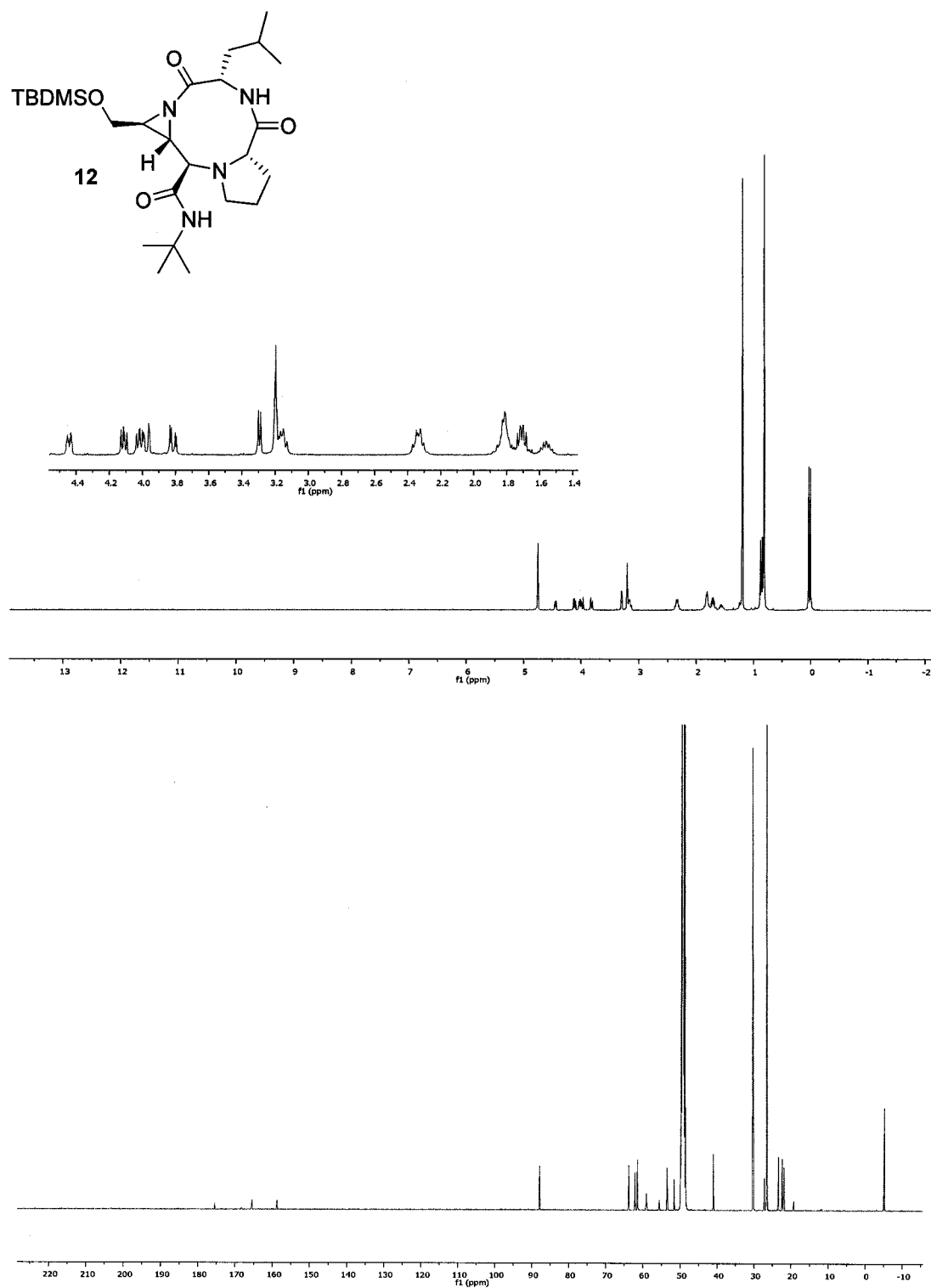
Figure 16. ^1\text{H} and ^{13}\text{C} NMR spectra for cyclic product 12.
