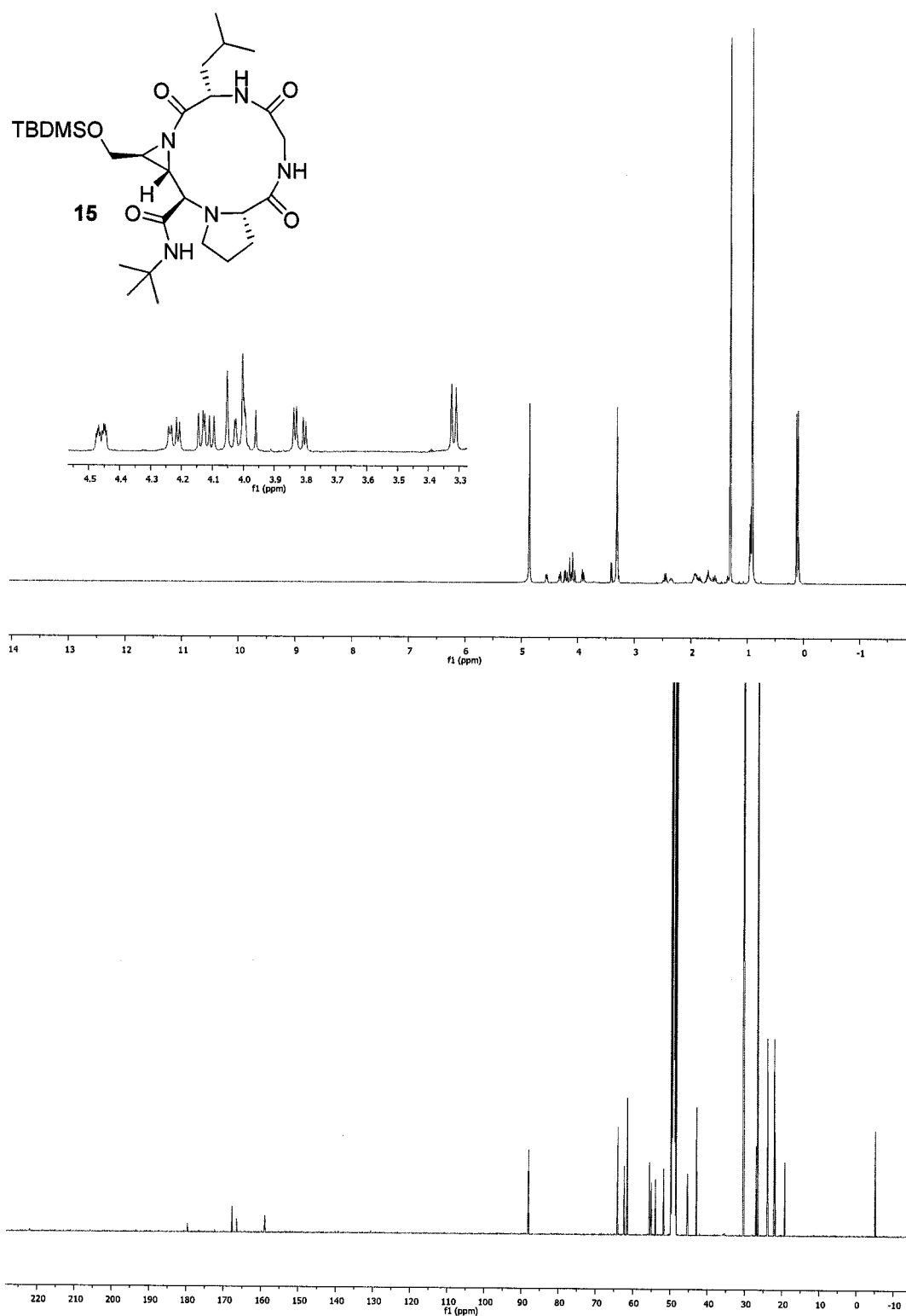
Figure 19. ^1\text{H} and ^{13}\text{C} NMR spectra for cyclic product 15 .
