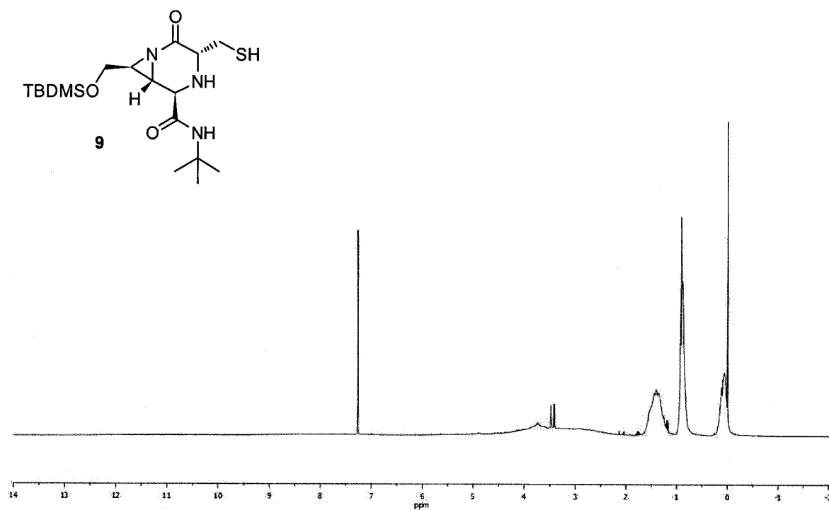
Figure 13. ^1\text{H} NMR spectrum for cyclic product 9.
