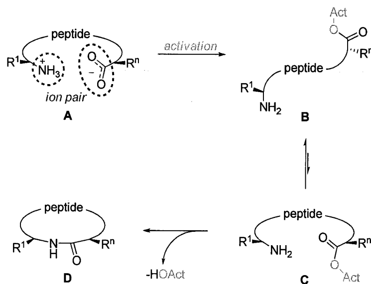
Scheme 1. A common peptide macrocyclization strategy.
