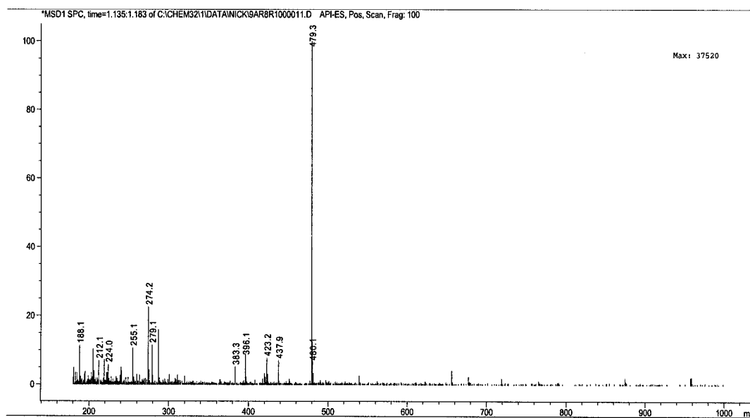
Figure 29. Crude LC-MS(ESI) analysis of isocyanide/amino aldehyde-mediated cyclization of Pro-Gly-Gly-Gly at 0.2M
