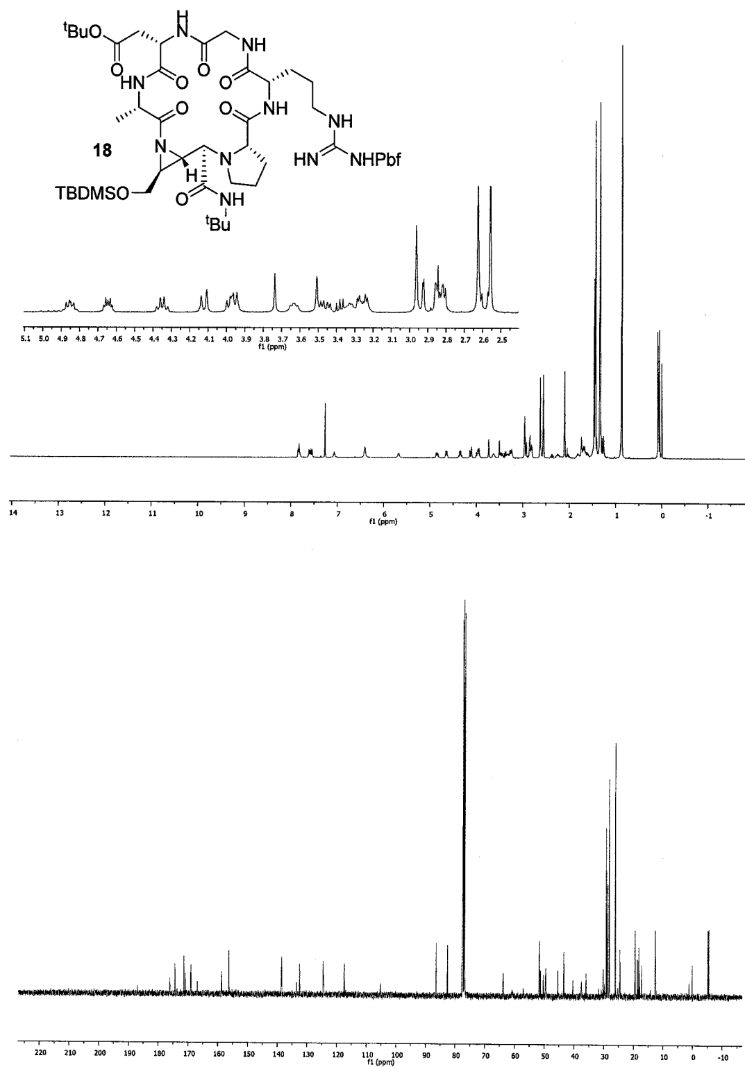
Figure 22. ^1\text{H} and ^{13}\text{C} NMR spectra for cyclic product 18 .
