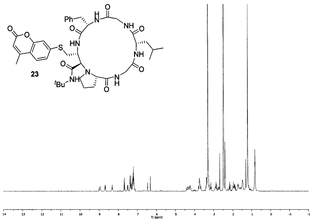
Figure 27. ^1\text{H} NMR spectrum for cyclic product 23 .
