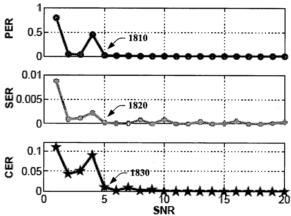
PER, SER, and CER of Normal transmissions under different SNR
