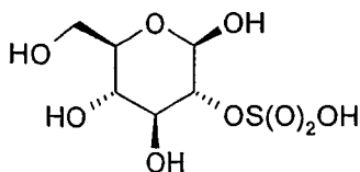
2-sulfuric acid- \beta -D-glucose
