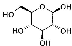
\beta -D-glucose
