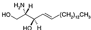
Sphingosine (also: trans-4-sphingenine) (also: (4E)-sphingenine) (also: (2S,3R,4E)-2-amino-4-octadecene-1,3-diol)
